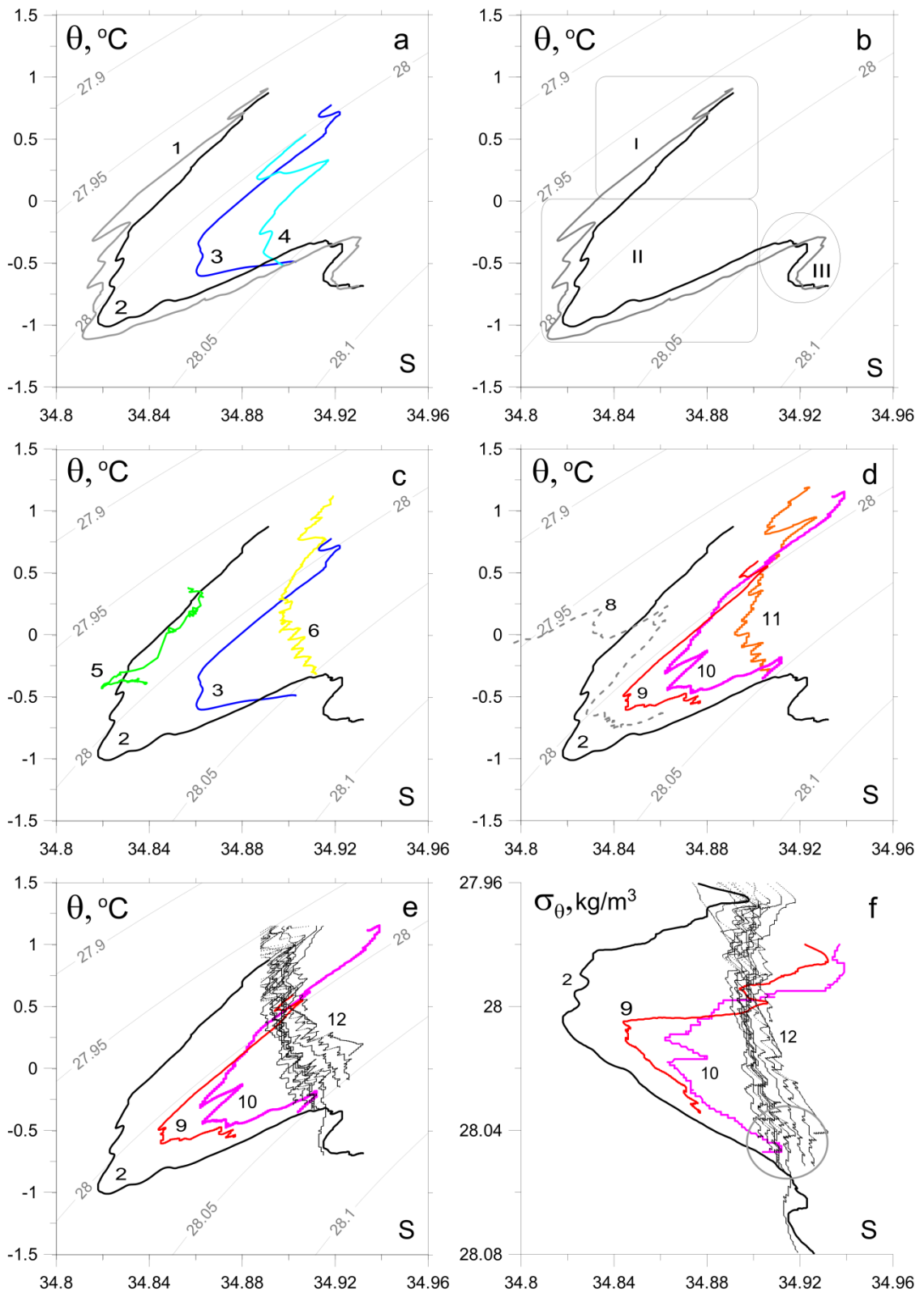
Fig. 8. Thermohaline indexes values of the BSBW and FSBW: a) based upon the CTD profiles, obtained in the St. Anna Trough (NABOS-09, section 82°N), curves 1–4 correspond to the stations (st.) 76, 78, 83 and 80, respectively; b) the same as “a” but only curves 1 and 2 are presented; regions I, II, III illustrate three different water masses in accordance with (Dmitrenko et al., 2015); for explanation see the text; c) based upon the section of PS-96, curves 5 and 6 corresponding to st. 32 and 42, respectively (depth range 600–1000 m), curves 2 and 3 are
