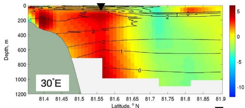
Figure 2. Temperature (contours, °C) and geostrophic velocity (colours, cm/s) relative to 0m reference level vs latitude and depth for the same NABOS-2006 transect at 30°E taken from Pnyushkov et al. (2015).
