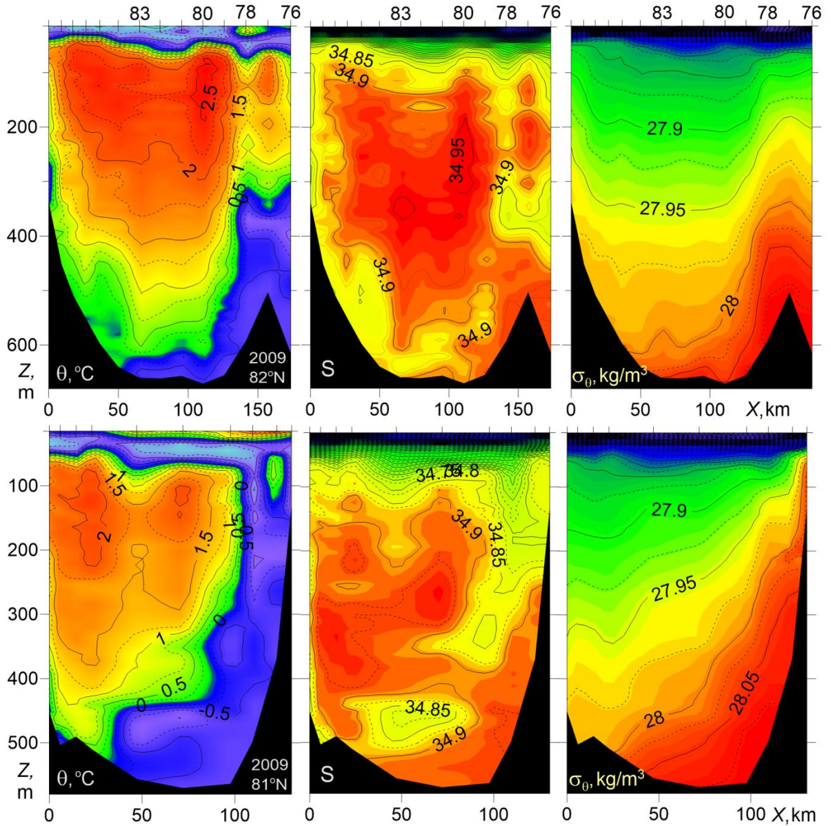
215 Fig. 3. Temperature \theta , salinity S , and potential density anomaly \sigma_\theta versus distance and depth for zonal transects across the St. Anna Trough at latitudes of 81°N (bottom, NABOS-2009), and 82°N (top, NABOS-2009). The X -axis is directed to the east.
