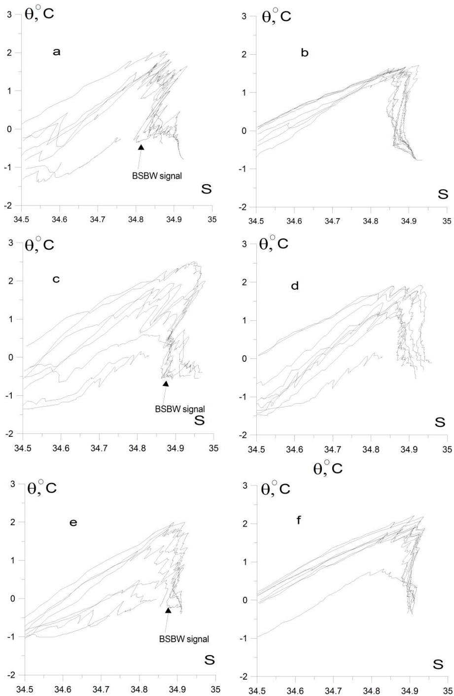
Fig. 9. \theta - S diagrams based on the CTD profiling : NABOS-05: (a) and (b), 103°E (a), 126°E (b); 430 NABOS-06: (c) and (d), 103°E (c), 126°E (d); NABOS-08: (e) and (f), 103°E (e), 126°E (f).
