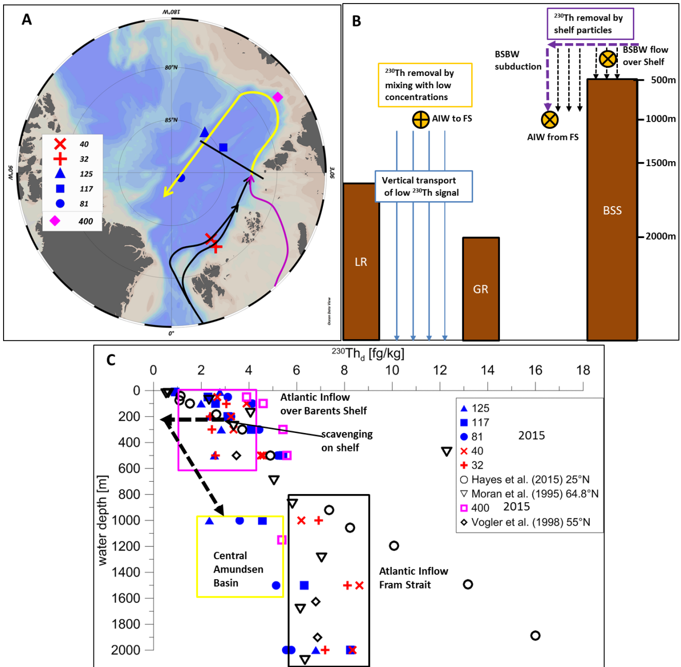
Figure 5: (A) Circulation pathways of Atlantic waters to the central Amundsen Basin. (B) Conceptual drawing of scavenging and mixing of water masses close to St Anna Trough (black line in A represents the section of B). LR = Lomonosov Ridge, GR = Gakkel Ridge, BSS = Barents Sea Shelf, FS = Fram Strait). (C) Development of dissolved ^{230}\text{Th} concentrations from the North Atlantic to the Amundsen Basin. Atlantic values: (open symbols, Hayes et al., 2015; Vogler et al., 1998; Moran et al., 1995) represented by a deep box flowing in through Fram Strait and a shallow box with lower activities flowing in over the Barents shelf and exposed to additional scavenging on the shelf (horizontal black arrow) before it is subducted and mixed with deeper Atlantic inflow to form the observed reduced concentrations in the central Amundsen Basin. Stations 32 and 40 (red) are from Gdaniec et al. (submitted).
