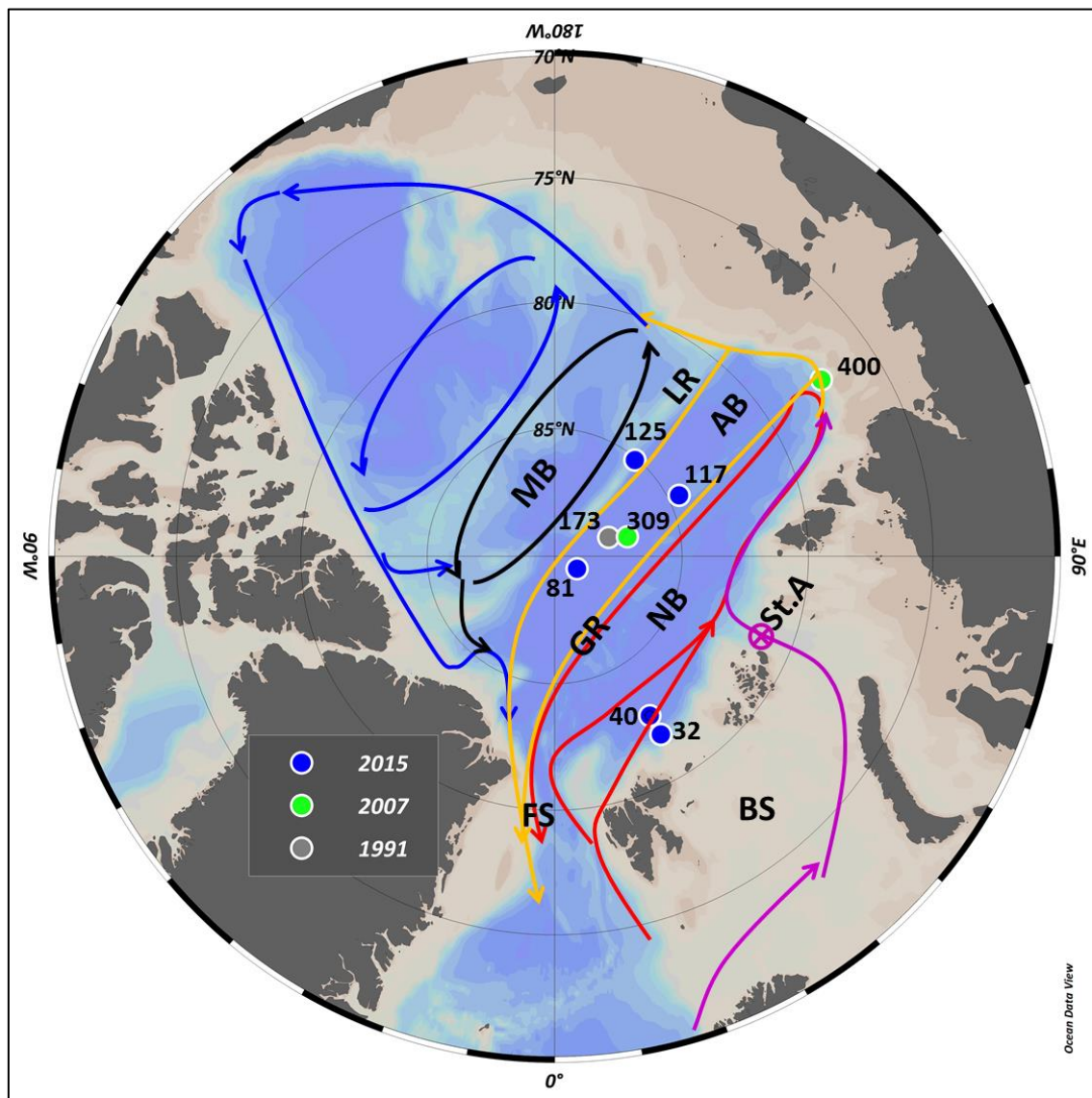
Figure 1: Map of the Arctic Ocean and station overview. AB = Amundsen Basin, NB = Nansen Basin, GR = Gakkel Ridge, MB = Makarov Basin. BS = Barents Sea, FS = Fram Strait, LR = Lomonosov Ridge, (X) = subduction at St. Anna Trough (St.A) with intermediate water circulation patterns after Rudels (2009). Red is the Atlantic inflow through Fram Strait (FSBW) and return flow through the Nansen Basin; purple is the inflow through the Barents Sea (BSBW). Atlantic layer circulation in the Amundsen Basin (orange), the Makarov Basin (black) and Canada Basin (blue) are indicated as arrows.
