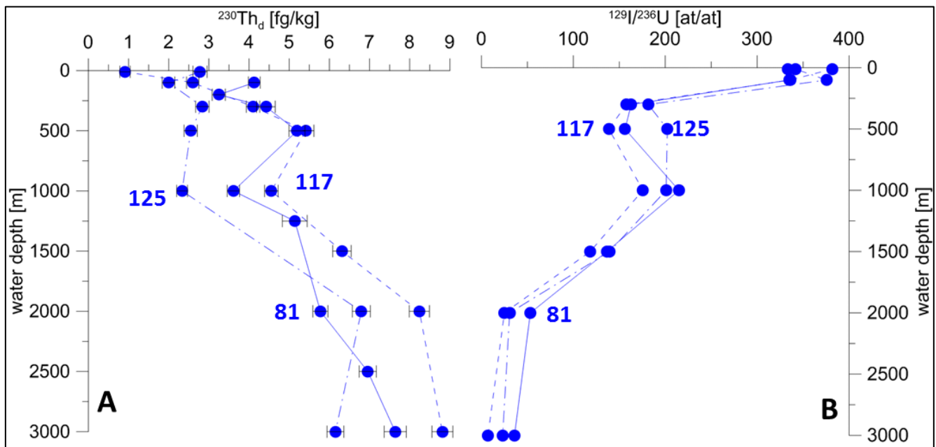
Figure 3: (A) Dissolved ^{230}\text{Th}_d . (B) ^{129}\text{I}/^{236}\text{U} (Casacuberta et al., 2018) from the Amundsen Basin, 2015
