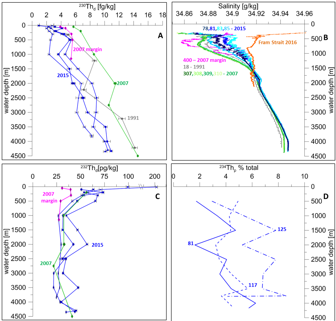
Figure 2: (A) Amundsen Basin dissolved ^{230}\text{Th} from 2015 in blue (81 = dots, 117 = squares, 125 = triangles), 2007 in green (309), 2007 margin in pink and 1991 in grey (173). (B) Amundsen Basin salinity profiles from 2015 (Rabe et al., 2016), 2007 (Schauer and Wisotzki, 2010), 1991 (Rudels, 2010) and Fram Strait 2016 (Kanzow et al., 2017). (C) Dissolved ^{232}\text{Th} from 2015 (81 = dashed, 117 = dashed dotted, 125 = solid) and 2007 (309 = green) and 2007 margin (400 = pink) (D) Particulate ^{234}\text{Th} from 2015 in percent of total ^{234}\text{Th} .
