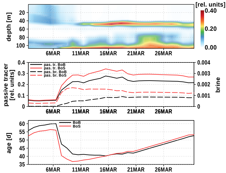
Figure 11. Time series of Bothnian Sea and Bay surface tracer at station 9 (Fig. 3). The upper panel shows the vertical distribution of Bothnian Sea surface water; the middle panel shows the concentrations of Bothnian Sea (red) and Bay (black) surface water, and the concentration of brine (dashed, right y-axis) in the bottom water at station 9; the lower panel shows the mean age of Bothnian Sea and Bay surface water in the bottom water at station 9.
