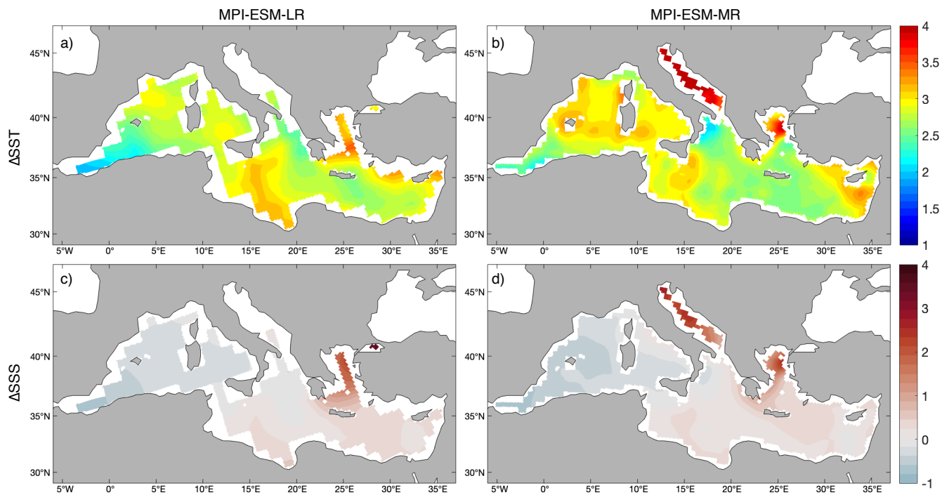
Figure 14: SST (in ^{\circ}\text{C} , upper row) and SSS (in psu, bottom) MPI-ESM-LR (left) and -MR (right) anomaly fields estimated as the difference between the average of the RCP8.5 projection (2070-2099) and present climate (1976-2005).
