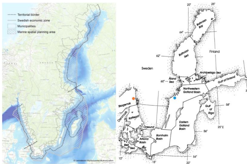
Figure 2: Left) Map of the SEEZ around Sweden in focus for this study. Right) Map of the considered water basins. The same basin terminology is used throughout the article. Credits to HELCOM (2018). The blue marker indicates the station at Landsort, while the orange marker points at the station of Väderöarna.
