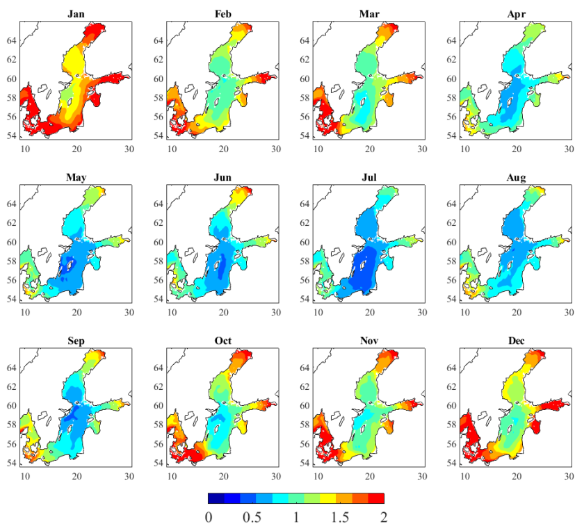
Figure 34: MSSHR_{m,10y} (Monthly maximum ranges [m] for each month over 10 years, 2007-2016, of re-analysis data). The red areas illustrate MSSHRs higher than about 1.8 m, up to 4 m.
