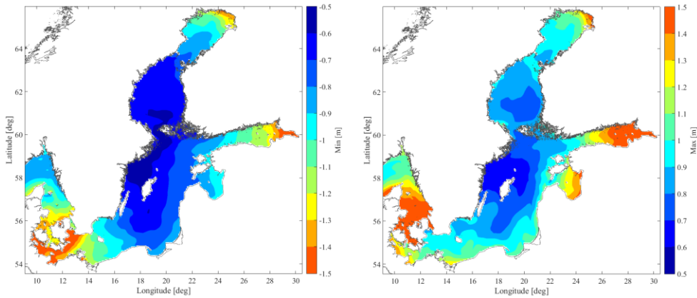
Figure 89: Lowest minima (left) and highest maxima (right) of the SSH_{th} during the period 2007 to 2016, after subtracting the mean value.
