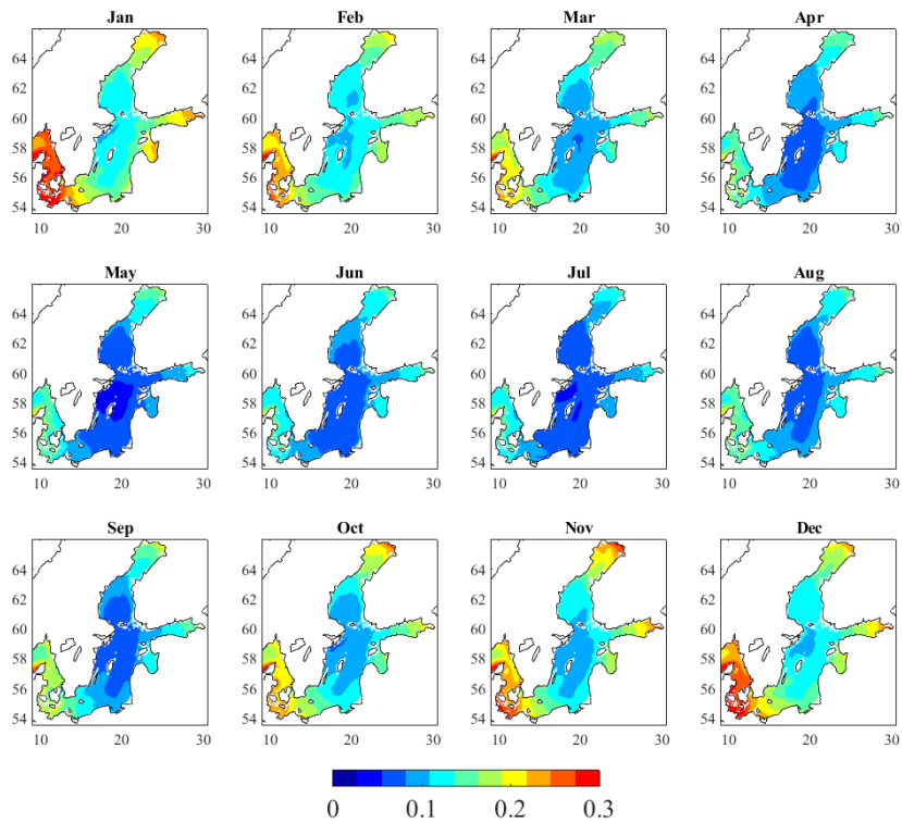
Figure 56: SD_{m,10y} (Monthly SD [m] for each month over 10 years, 2007-2016, of re-analysis data).
