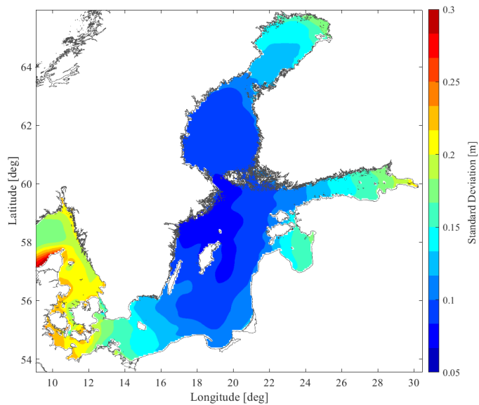
Figure 67: SD_{10y} (Decadal SD of the SSH_h over the 10-year window). The colour scale is different from the one in Fig. 5-6 for ease of readability and visualization.
