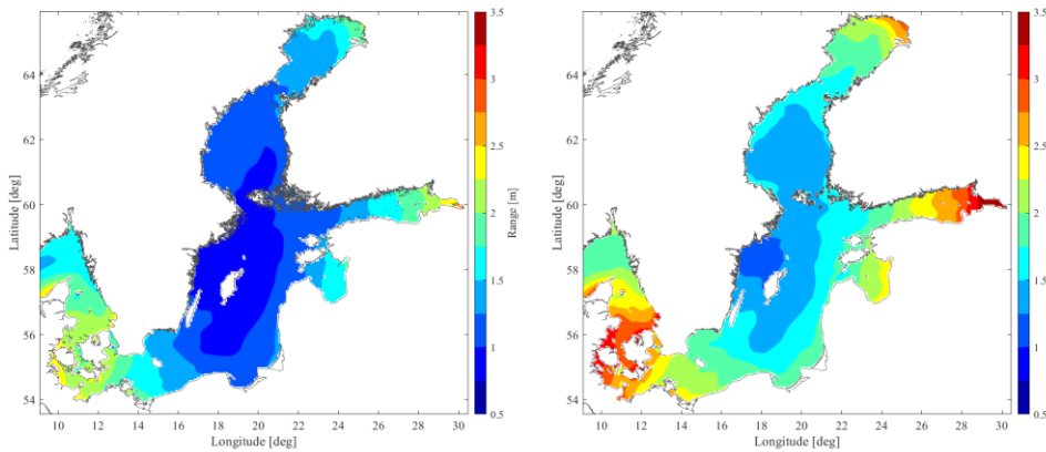
Figure 45: Left) Average MSSHR y (average annual maximum ranges over the 10-year window). Right) MSSHR 10y (decadal maximum ranges over the 10-year window). The colour scale is different from the one in Fig. 3-4 for ease of readability and visualization.
