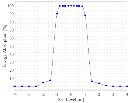
Figure 78: Normalized annual energy absorption as a function of the SL for a L12 Uppsala WEC and for a sea state characterized by H_s = 1 m and T_e = 5 s. The markers indicate the results of the hydro-mechanic simulations, while the solid line serves as a guide to the eye. Adapted from Castellucci et al. (2016).
