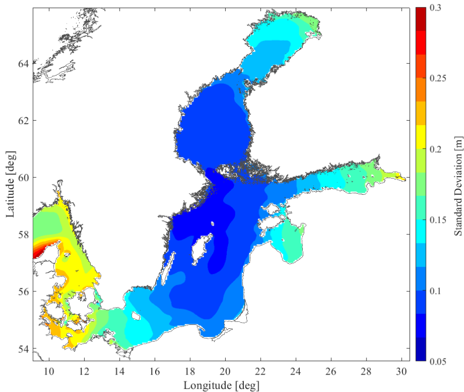
Figure 6: SD_{10y} (SD of the MSSH_y over the 10-year window). The color scale is different from the one in Fig. 5 for ease of readability and visualization.
