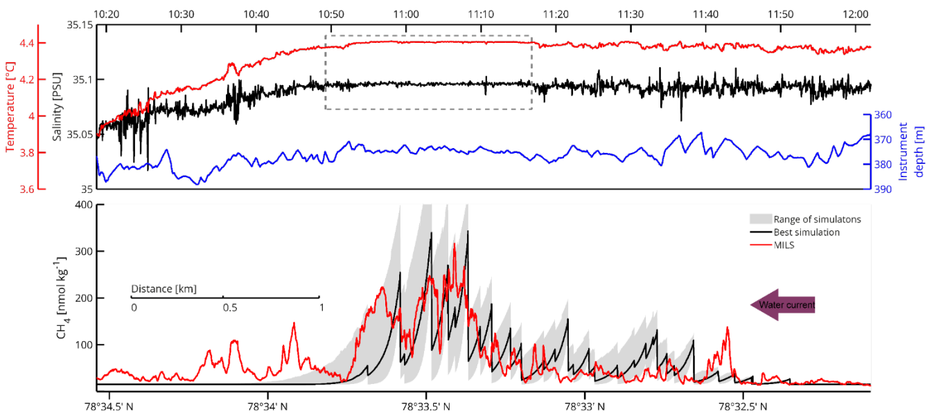
310 Figure 6. Water properties and comparison between modelled and measured dissolved \text{CH}_4 concentrations along line 3. Top panel shows temperature and salinity data together with the depth of the towed instruments. The dashed-line box highlights the area of intense mixing. In the lower panel, the red line shows the dissolved \text{CH}_4 measured by the MILS. The grey area indicates the range of \text{CH}_4 concentrations from the 2D model simulations. The black line depicts output of the model simulation with the best match 315 with the measured concentrations.
