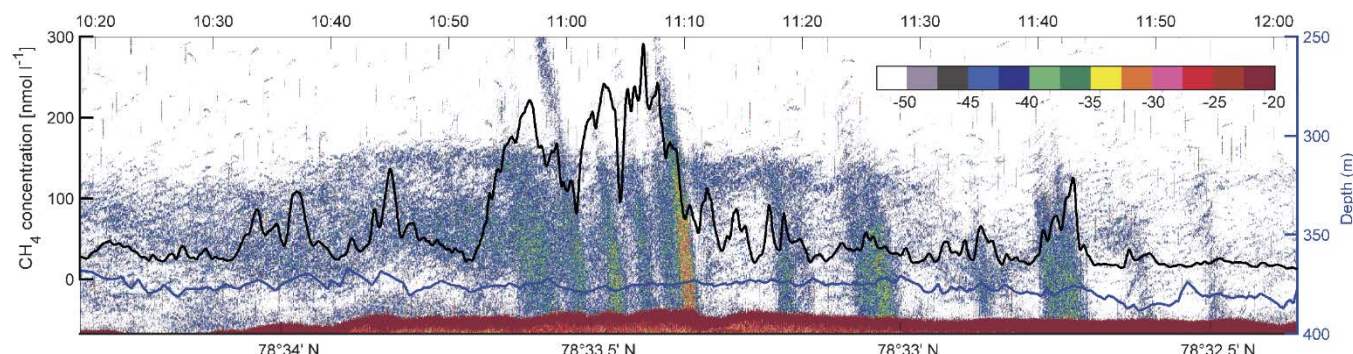
Figure 5. Towed MILS data overlaying echo-sounder data. The black line shows the CH 4 concentration along line 3 (see Fig. 1 for location) at ~15 m from the seafloor. The blue line indicates the depth of the probe. The echogram, displaying TS values (colour bar shows intensity (-dB)) from the 38 kHz-channel of the EK60, is shown in the background.
