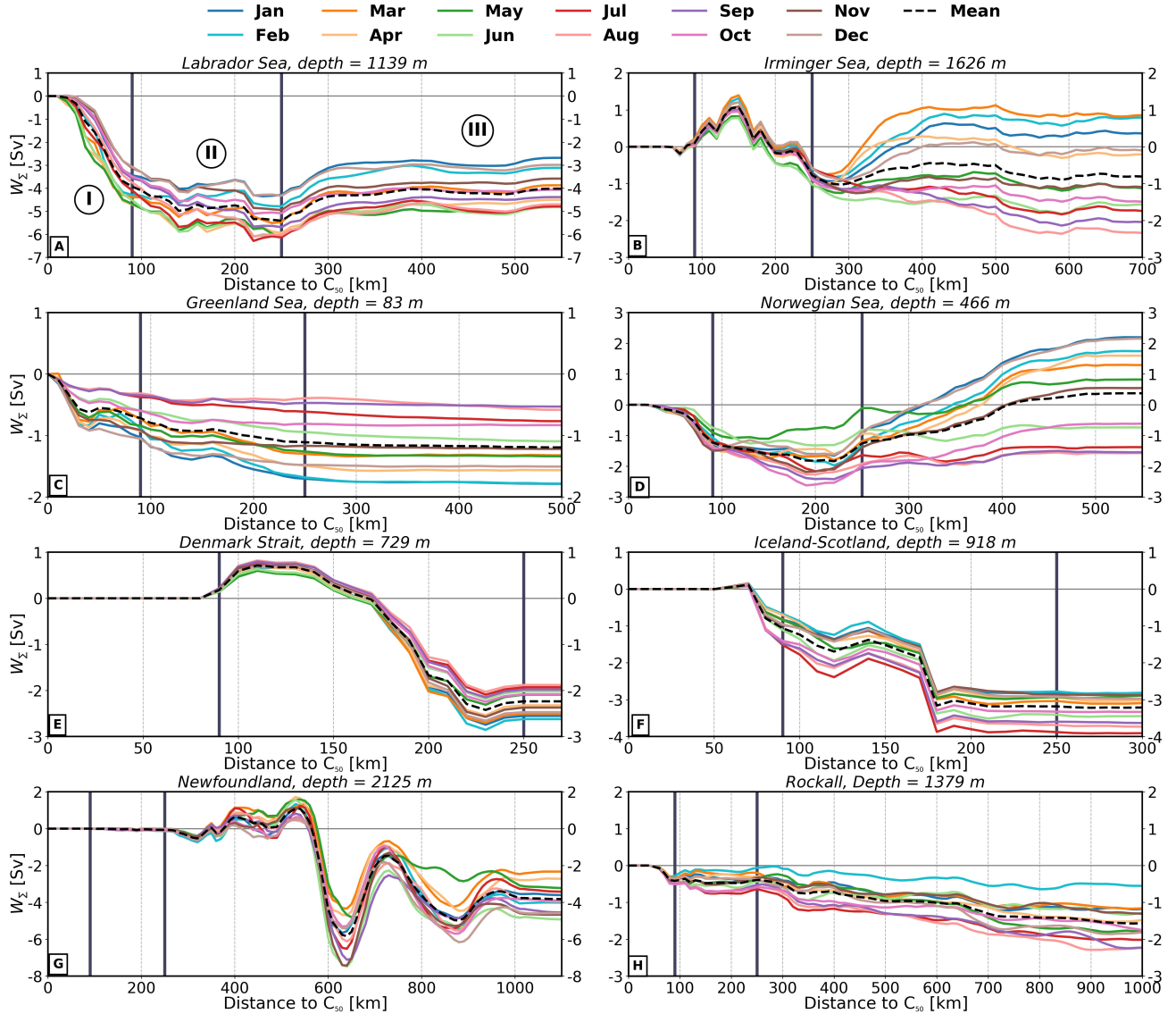
Figure 8. Accumulated net vertical transport ( W_\Sigma ) with respect to the distance to the closest bathymetric contour of 50 m ( C_{50} ). Distances are shown in Fig. 4 (inset map). Annual (dashed black line) and monthly mean (colored lines) curves are depicted for the regions defined in Fig. 6. The accumulated W_\Sigma has been calculated at the depth of minimum time-mean W_\Sigma ( z_{\min} ), which differs for each region (see Table 2 and plot title). The bounds separating the sinking regimes (I-II-III) proposed in Fig. 4 (90 km, 250 km) are indicated with thicker solid vertical lines. Note the differences in the horizontal and vertical scales in the plots.
