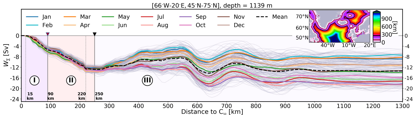
Figure 4. Cumulative net vertical transport ( W_\Sigma ) at a depth of 1139 m (in Sv) as a function of the distance from the bathymetric contour of 50 m depth referred to as C_{50} (inset map in Fig. 4). If the grid cell bathymetry is shallower no value is added. The dashed black line shows the annual mean. Monthly values of the 15-year simulation are shown in light gray, colored lines indicate the monthly climatology. The regimes of sinking are indicated by roman numbers I–II–III, and the separation lines between them are also denoted by a brown and a black triangle and by contours in the same color in the inset figure.
