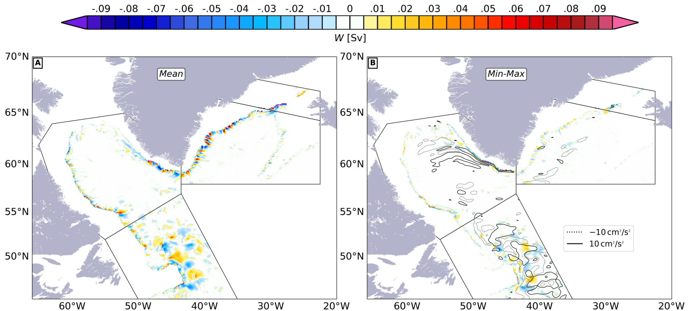
Figure 10. (A) Composite map of mean vertical transport ( W ) for the western regions of study (defined in Fig. 6) at the corresponding depth of minimum time-mean W_\Sigma , which differs for each region according to Table 2. (B) Same as (A) but now the mean W (shading) and EKE (black contours, see legend) at the month of minimum W_\Sigma minus the mean W at the month of maximum W_\Sigma is plotted. These months of minimum and maximum sinking also change for each region according to Table 2. Units of W in Sv and of EKE in \text{cm}^2 \cdot \text{s}^{-2} .
