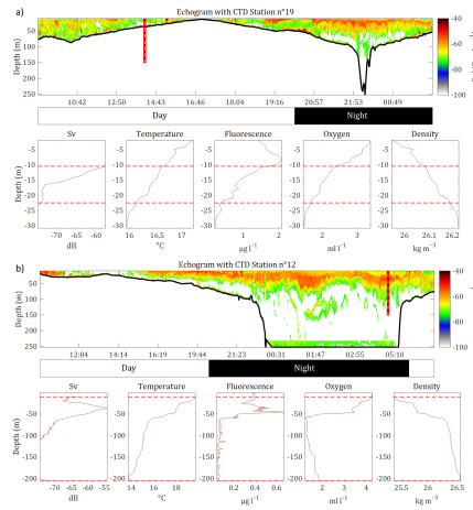
Fig. 1: Echograms and associated vertical acoustic profiles as well as physico-chemical parameters (CTD data) for two example stations: (a) station 19 in the 'inshore area' and (b) station 12 in the 'offshore area'. For both (a) and (b), top panels are echogram data collected along the transect (nm), whereas the bottom panels depict acoustic and environmental data (depicted by the red vertical line in top panels). Environmental data for the sound scattering layer (SSL) collected at the stations at the time depicted by dotted vertical lines. Data represent mean conditions for the station collected within an area of 0.1 nm area around the station: acoustic volume backscattering strength ( S_v ) SSL, temperature profile SSL, CHL profile SSL, oxygen profile SSL, and density profile SSL.
