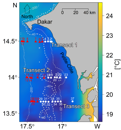
Fig. 1: Location of the survey area off the southern Senegalese (West African) coast. The hydroacoustic survey was conducted with FRV Antea (RD) from Dakar (Cap Vert peninsula in the north) to the northern border of Gambia (horizontal black line). CTD-probes collected data at stations along three transects perpendicular to the coast (R1 to R3). Sea surface temperature (SST, °C) were averaged over the three days of CTD sampling from the 6-8 March 2013. Stations of Group 1 (blue circles) occurred in the inshore zone, whereas stations of Group 2 (red triangles) were situated more offshore.
