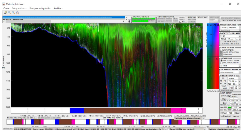
Figure 1 revision: [only for referee] ; representation of an ECOAO echogram (from 06 h -07 h ) at three frequencies. Each frequency (here 38, 70 and 120 kHz) was scaled from 0–255 and assigned a colour RGB value based on its frequency. This method allow to clearly observe that the signal is mainly associated to 38 kHz and allow to find the same SSL shape than combined frequency.
