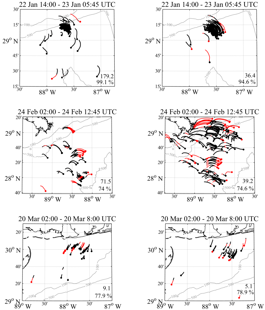
Figure 8: Drogued (left) and undrogued (right) drifter trajectories during the hours of analysis for each high wind event. Time periods over which the total velocity deconstructions were calculated are shown in each title. Portions of the trajectories shown in black (red) depict segments which overlap (do not overlap) spatially with each respective Eulerian velocity field in Fig 4. (Top) the total number of retained trajectory data points, defined as number of drifter days given 15-minute time steps, and (bottom) the percentage of coverage between trajectories and each respective Eulerian velocity field in Fig.4 are listed within each plot. Trajectories missing head markers are a result of either drogue loss or lost GPS transmission during the experiment.
