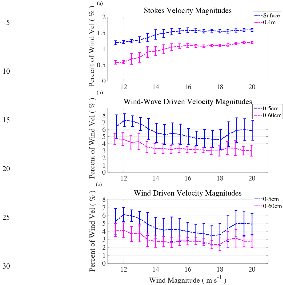
Figure 13: Average velocity magnitudes at drifter locations during periods of high wind binned by UWIN-CM wind magnitude on 0.5 \text{ m s}^{-1} intervals. (a) UWIN-CM Stokes drift velocity magnitude at the surface (0 m) and at 0.4 m depth. (b) Velocity magnitude of drogued and undrogued drifters after the subtraction of the pre-existing circulation estimate. (c) Velocity magnitude of the purely wind-driven component of the drifter velocities. All error bars show \pm one standard deviation within each bin. Data bins omitted in Figure 9 are also excluded.
