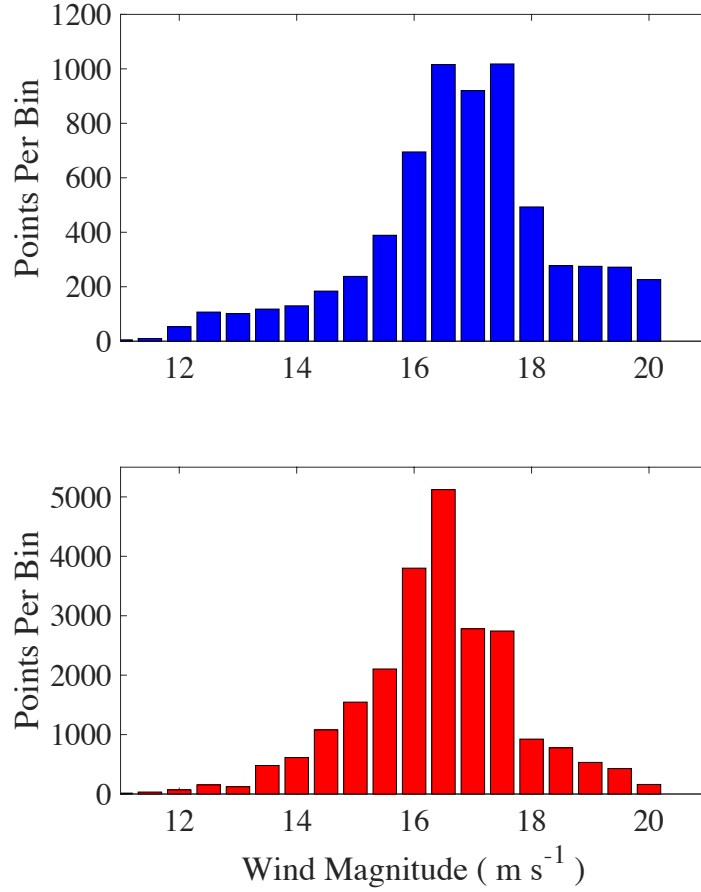
Figure 11: Number of undrogued (top) and drogued (bottom) drifter positions where the velocity deconstruction was performed, binned by wind velocity magnitude on 0.5 m s -1 intervals. Point velocity measurements calculated from drifter trajectories that do not coincide spatially with available data in the pre-existing circulation velocity fields are not included.
