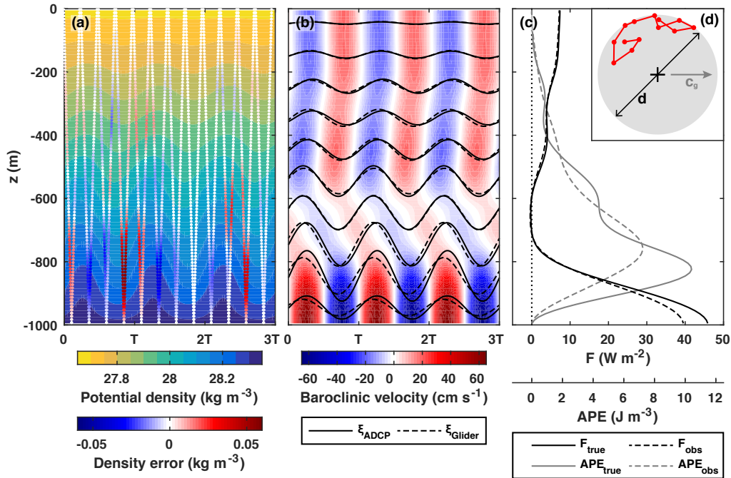
Figure 7. (a) Potential density for an idealised M_2 multi-mode internal tide overlaid with the error in measured density due to imperfect co-location of a glider and ADCP. The x-axis is time in M_2 cycles. Positive error indicates an overestimation of density. (b) Baroclinic velocity (colour) for the same idealised internal tide overlaid with vertical isopycnal displacement at the ADCP ( \xi_{\text{ADCP}} , solid black lines) and calculated from measured density ( \xi_{\text{Glider}} , dashed black lines) every 100 m. (c) ‘True’ and ‘observed’ internal tide energy flux (black) and available potential energy (grey). (d) Location of the pseudorandomly distributed glider path (red) relative to the ADCP (black cross). The diameter of the watch circle, d = \lambda/4 , where \lambda = 80 km is the mode-1 horizontal wavelength. c_g is the direction of wave propagation.
