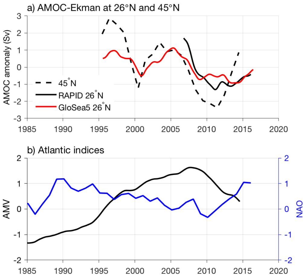
595 Figure 6 (a) AMOC anomalies from RAPID at 26°N (black, Sv), 26°N GloSea5 reanalysis (red, Sv), AMOC 45°N (black dashed, Sv). b) The AMV (black) and NAO (blue). The AMV has been decadal low-pass filtered, with a 5-year low-pass filter applied to the NAO time series. The Ekman transport has been removed from the AMOC time series.
