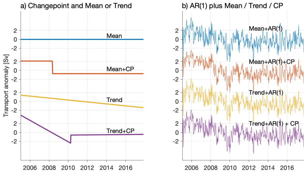
590 Figure 5 Change point analysis of the AMOC-Ekman time series. In panel (a), only a mean or a trend, with or without a change point are fit. In panel (b), an AR(1) is also fit. The model with the best overall fit is the Mean + AR(1) + CP model (red, right) according to the AIC (see Table 2), indicating that the time series can best be explained by an AR(1) time series with a change in the mean in 2008.
