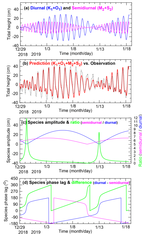
Fig. 2. Figure 10. Time series (29 December 2018 to 18 January 2019) of (a) predictions of the diurnal (K1+O1) tides (blue line) and the semidiurnal (M2+S2) tides (magenta line) for JBARS; (b) their combined
