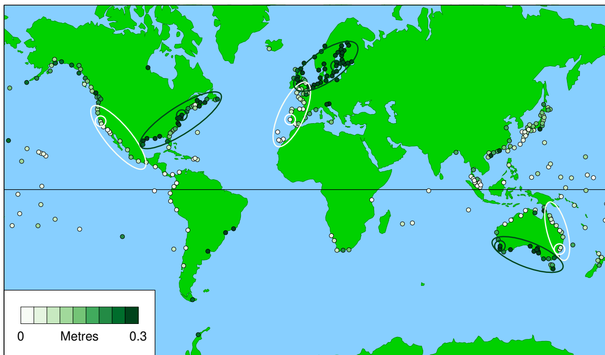
Figure 2. Averaged first metric, which is height of highest observed sea level above observed maximum on day of highest predicted tide for the year, for daylight days ( o_d(I_{od}(j,k),j,k) - o_d(I_{pd}(j,k),j,k) ), averaged over all valid years, j . The large white and dark green circles indicate the records for the results shown in Figs. 7, 8 and 9. The white and dark green ellipses indicate the regions discussed in Section 4.
