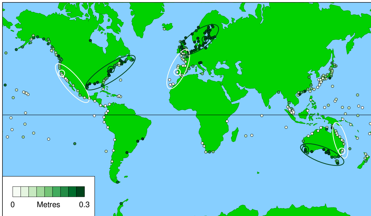
Figure 2. Averaged first metric , which is height of highest observed sea level above observed maximum on day of highest predicted tide for the year, for daylight days ( o_d(I_{od}(j, k), j, k) - o_d(I_{pd}(j, k), j, k) ), averaged over all valid years, j . The large white and dark green circles indicate the records for the results shown in Figs. 7, 8 and 9. The white and dark green ellipses indicate the regions discussed in Section 4.
