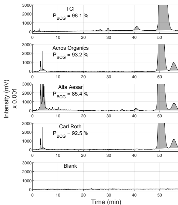
Figure 2. Analytical HPLC chromatograms of unpurified BCG from different vendors with their P_{\text{BCG}} and a chromatogram from a solvent injection without BCG (Blank). All peaks are highlighted with gray background color.
