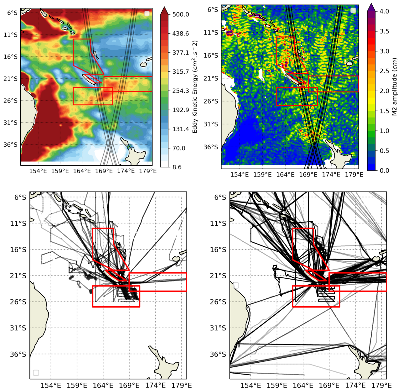
Figure 2. Regions of study (red boxes) around New Caledonia: Eddy Kinetic Energy estimated using DUACS (top left), M2 coherent internal tide estimated from satellite altimetry (top right), SADCp (bottom left) and TSG (bottom right) sections performed in the South West Pacific.
