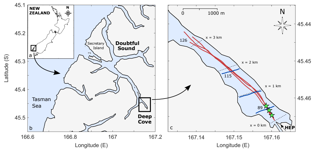
Figure 1. Location map of (a) New Zealand with the Fjordland region highlighted, (b) Doubtful Sound identifying the location of (c) Deep Cove showing the repeated across-channel (blue) and along-channel (red) vessel transects taken on three separate days in March 2016. The sampling started at the tailrace exit point and continued downstream towards the seaward end of Deep Cove. The mooring locations (stars) are shown. The arrow at the bottom right of (c) indicates the tailrace inflow from the Manapouri hydroelectric power station (HEP) discharged into the head of Deep Cove. The dashed lines across the fjord are reference distances from the tailrace discharge point ( x = 0, 1, 2, 3 km) and are referenced in the text and in other figures.
