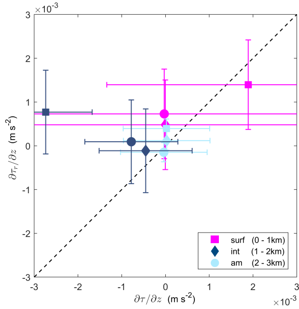
Figure 10. Directly observed internal stress divergence from microstructure profiler ( \partial\tau/\partial z ) compared to control-volume derived residual internal stress divergence ( \partial\tau_r/\partial z ). The terms are averaged over each layer: surface (pink), interface (dark blue), and ambient (light blue); and over each 1 km region from the tailrace discharge point: 0 - 1 km (square), 1 - 2 km (diamond), and 2 - 3 km (circle). The errorbars indicate one standard deviation for each term.
