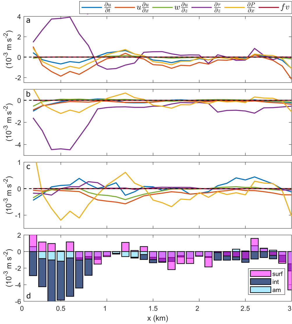
Figure 9. The individual and sum of all the layer-averaged terms in the along-channel momentum budget. The budget terms were averaged over the depth of (a) the plume ( 0 \leq z < 2 m), (b) the interface ( 2 \leq z < h m), where h is defined in Fig. 6b, and (c) the ambient below the surface layer ( h \leq z < 10 m). (d) The sum of all the layer-averaged momentum components within the surface (pink) and interfacial (dark blue) layers, and the ambient (light blue). Horizontal dashed lines indicate zero, where the budget is completely balanced.
