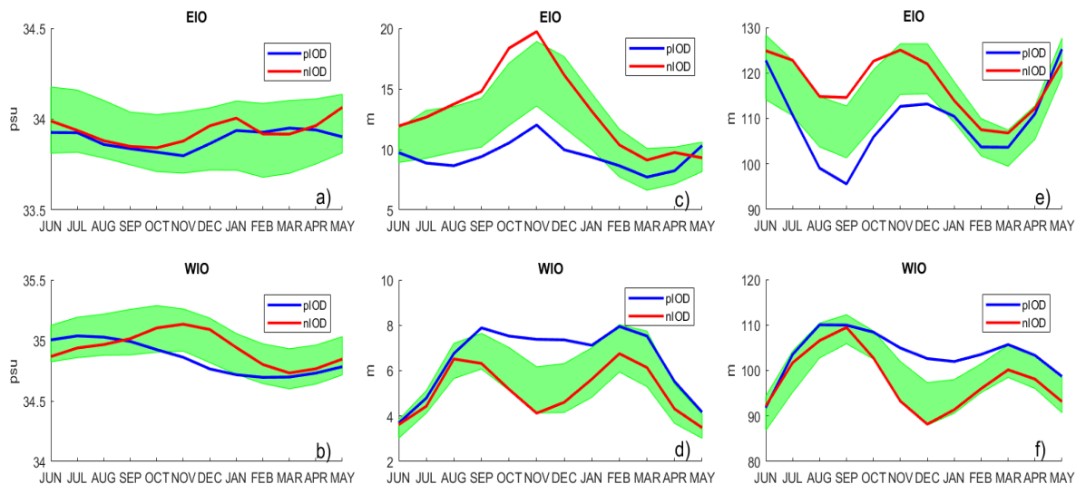
458 459 Figure 9. The compositing seasonal variations of SSS (a, b; unit: psu), BLT (c, d; unit: m) and the thermocline 460 depth(e, f; unit: m) in the IOD events during the period of 1980-2015 averaged by the areas of the eastern TIO (EIO, 461 85°E-100°E, 12°S-5°N) and the western TIO (WIO, 55°E-75°E,12°S-5°N), separately.The blue line represents 462 composite in the positive IOD events and the red one represents that in the negative IOD events and the green shaded 463 area represents the 95% Monte-Carlo significance level.
