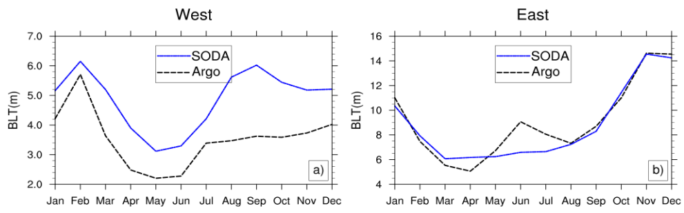
414 Figure 2. Seasonal cycle of the region-averaged BLT for SODA and Argo: a) the western TIO (55°E- 75 °E, 12°S- 415 5°N), and b) the eastern TIO ( 85°E - 100 °E, 12°S - 5°N).
