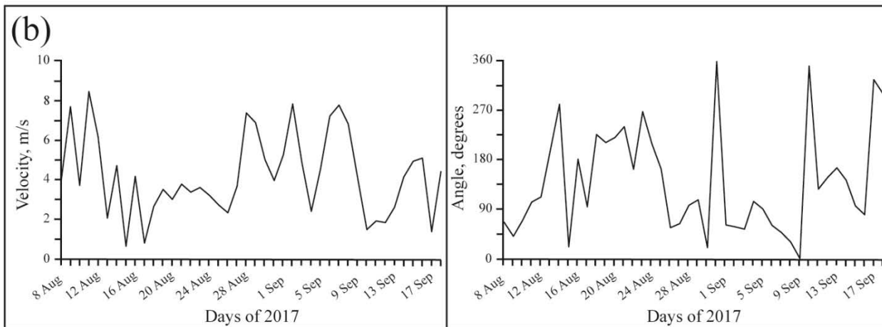
Figure 4: Average wind forcing (arrows) and sea level pressure (color) during 8-21 August (top left), 22 August – 3 September (top right), and 4-18 September 2017 in the western part of the Laptev Sea (a). Daily average wind speed (left) and direction (right) during 8 August – 18 September 2017 (b). Wind data were obtained from the ERA5 atmospheric reanalysis.
