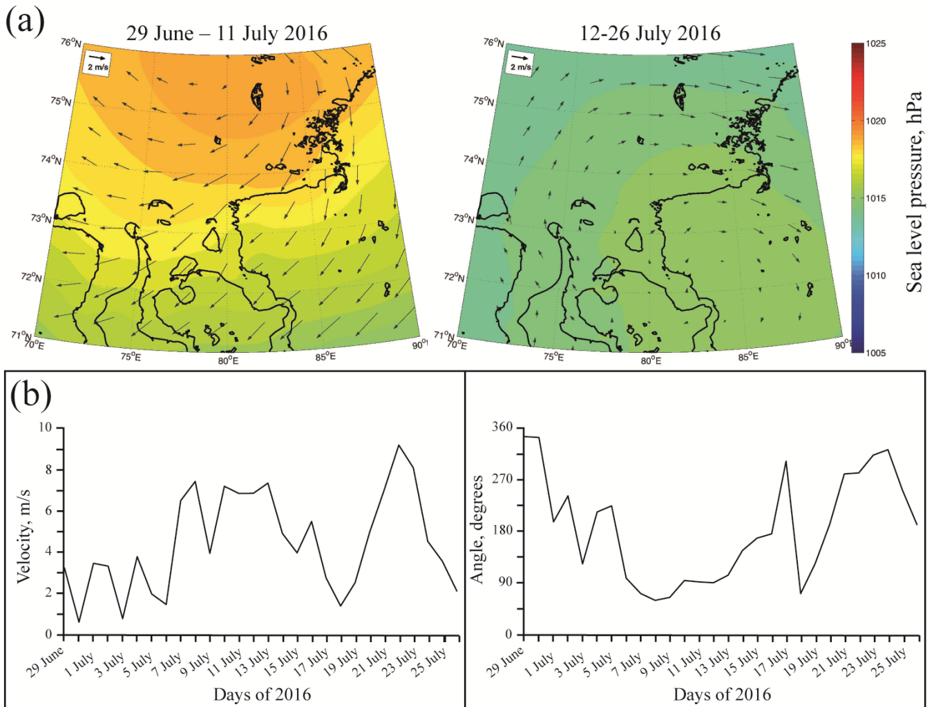
Figure 3: Average wind forcing (arrows) and sea level pressure (color) during 29 June – 11 July (left) and 12-26 July 2016 (right) in the central part of the Kara Sea (a). Daily average wind speed (left) and direction (right) during 29 June – 26 July 2016 (b). Wind data were obtained from the ERA5 atmospheric reanalysis. 195
