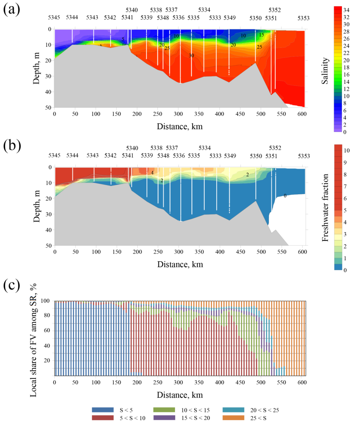
245 Figure 5: The vertical salinity structure (a), distribution of freshwater fraction (b), local shares of freshwater “volume” (FV) among salinity ranges (SR) in water column (c) along the ship track in the Yenisei Gulf and the adjacent shelf of the Kara Sea on 24-26 July 2016.
