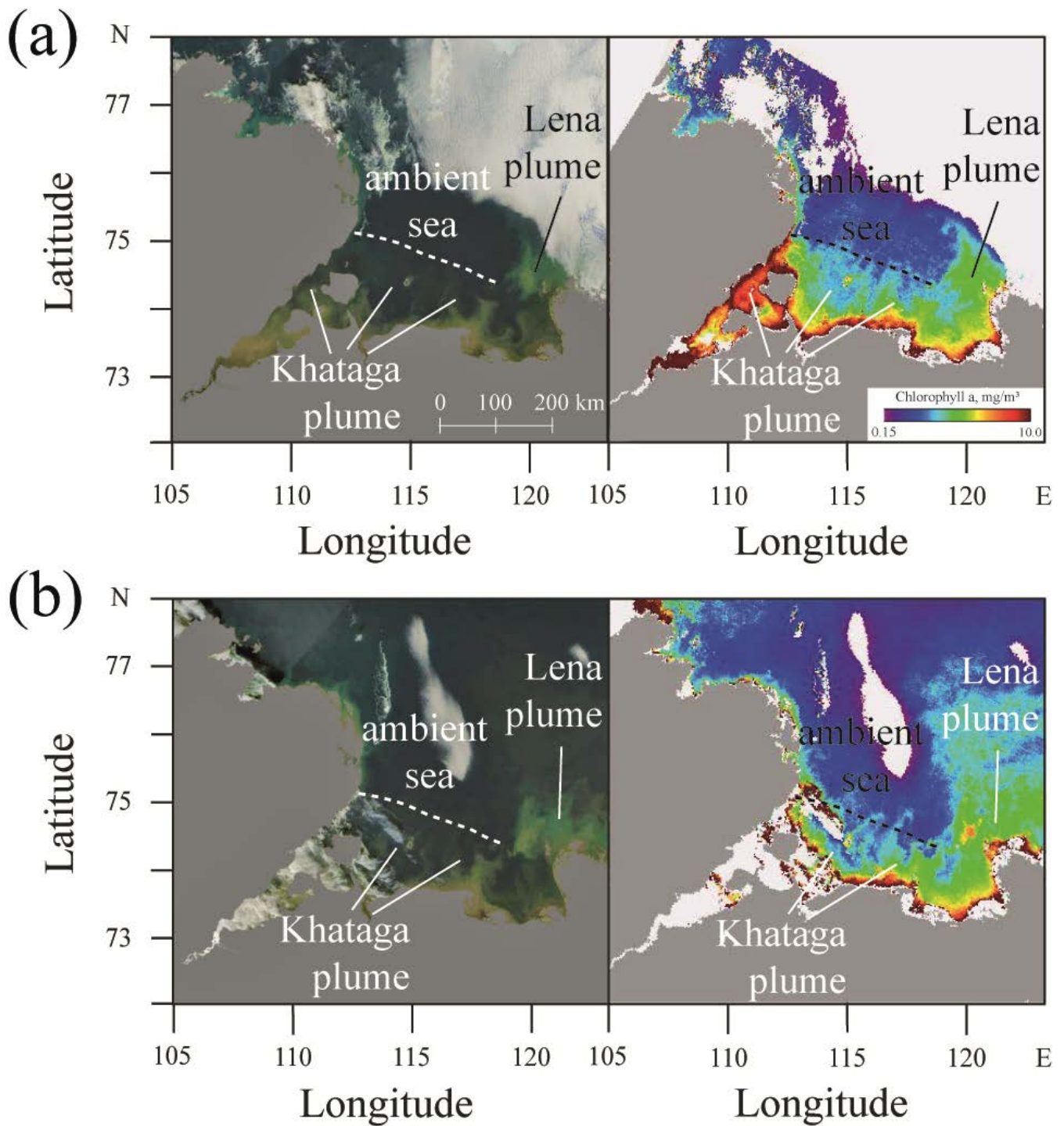
345 Figure 9: Corrected reflectance (left) and concentration of chlorophyll-a (right) from MODIS Terra satellite images of the western part of the Laptev Sea acquired on 23 September (a) and 25 September (b) 2000.
