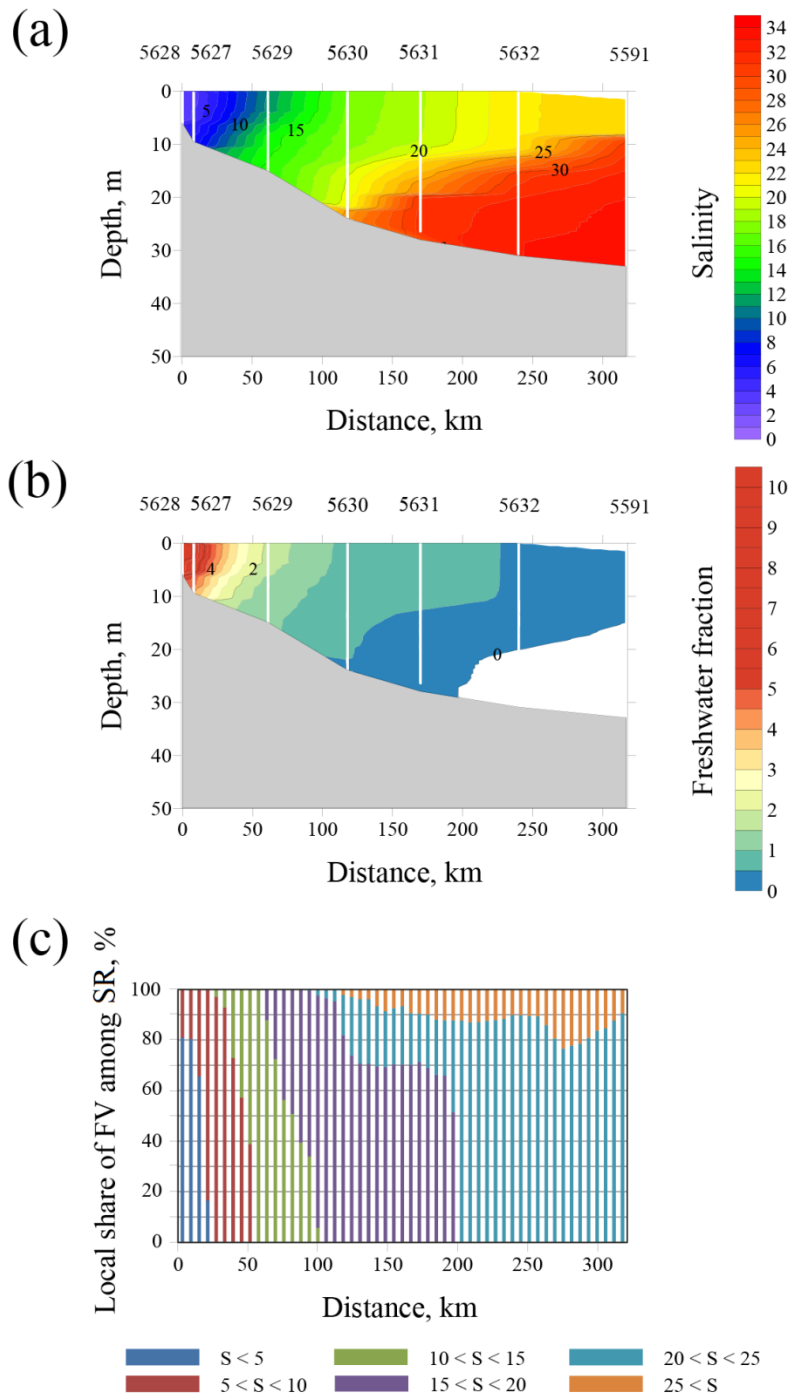
Figure 6: The vertical salinity structure (a), distribution of freshwater fraction (b), local shares of freshwater “volume” (FV) among salinity ranges (SR) in water column (c) along the ship track in the Khatanga Gulf and the adjacent shelf of the Laptev Sea on 17-18 September 2017.
