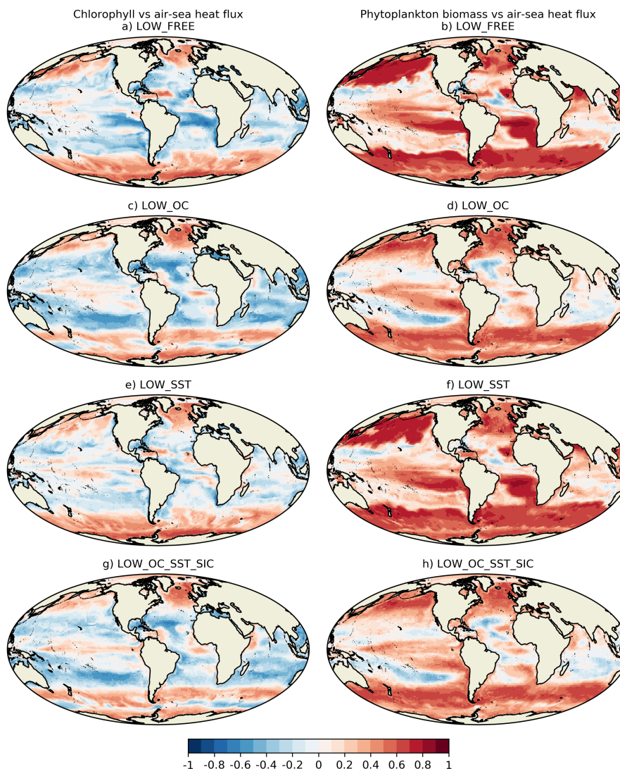
Figure 7. Maps of correlation between surface chlorophyll and net air-sea heat flux (left column) and surface phytoplankton biomass and net air-sea heat flux (right column), covering 1998–2010 for a selection of runs.
