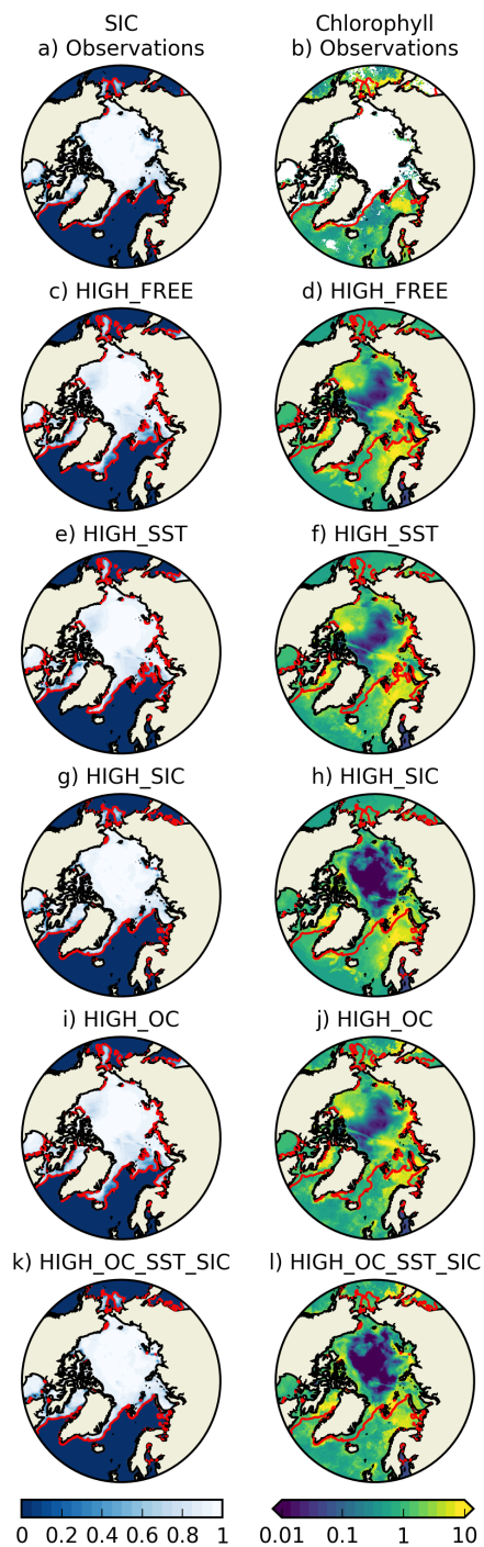
Figure 5. SIC (left column) and surface chlorophyll (right column) for 17–24 May 2010, from observed (a-b) and modelled (c-l) fields.
