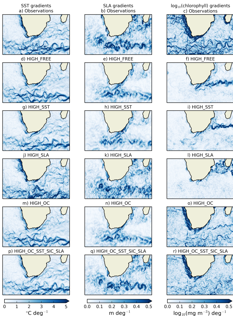
Figure 4. Observed and modelled gradients in the Agulhas Current region for December 2010.
