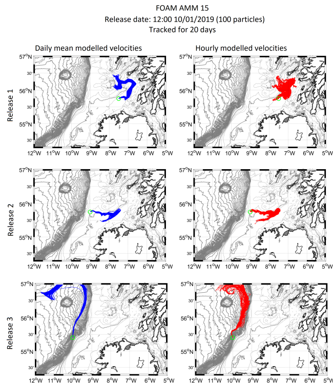
Fig. 1. Test particle releases into daily mean (left) and hourly (right) AMM15 model flow fields at 20 m depth.
