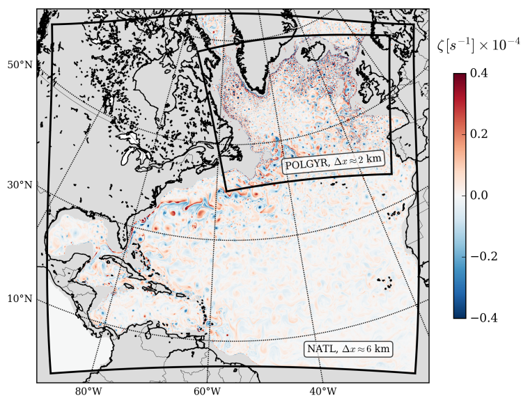
Figure 1. Snapshot of the relative vorticity at 500 m depth in the North Atlantic in the NATL simulation. The NATL grid ( \Delta x \approx 6 km) covers most the North Atlantic, and the POLGYR grid (smaller rectangle, \Delta x \approx 2 km) covers the subpolar gyre.
