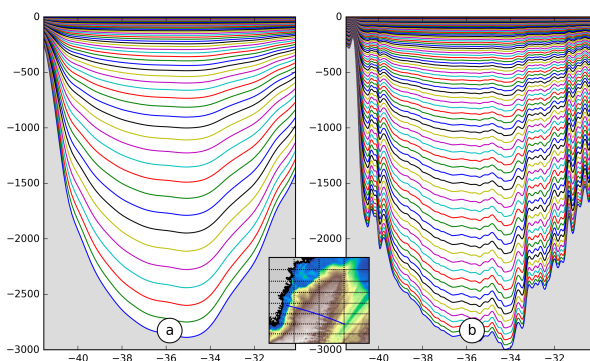
Figure 2. Depths of the model vertical \sigma -levels along a section of the Irminger Basin for (a) the 6-km simulation (NATL), and (b) the 2-km simulation (POLGYR).
