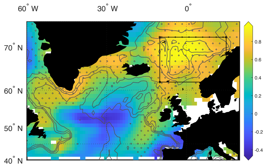
Figure 8. Correlation analysis between the Leading mode of variability of the deseasonalized (no trend removed) and annually-averaged temperature anomalies at 100 m in the eastern Nordic Seas (cf. left panel of Fig. 7) against every grid point of that in the North Atlantic using EN4. The black box encloses the area for the eastern Nordic Seas used here. Circles indicate significance at the 95% confidence level. Gray contours are bathymetry.
