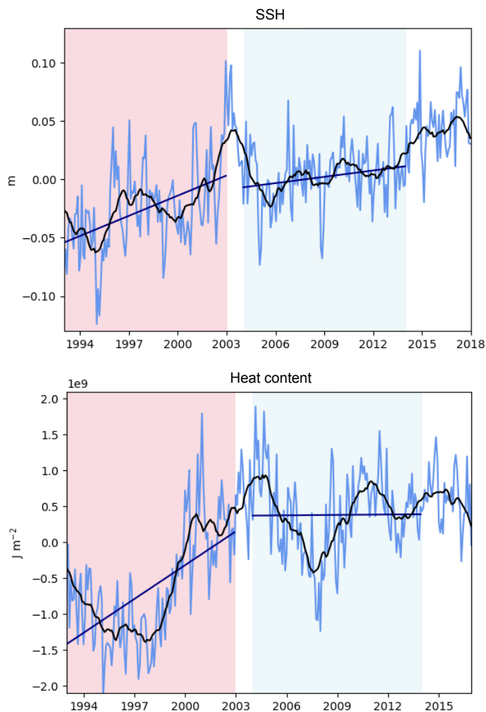
Figure 4. Upper panel: Monthly (light blue) and lowpass filtered (black) SSH [m] from 1993-2017 averaged over the AW area (see fig 1). The SSH has been deseasonalized. In dark blue are the linear trends of the SSH for the two periods 1993-2002 and 2004-2013. Lower panel: Monthly (light blue) and lowpass filtered (black) heat content in the upper 657 m of the AW area [ \text{J m}^{-2} ]. The heat content has been deseasonalized. In dark blue are the linear trends for the two periods 1993-2002 and 2004-2013.
