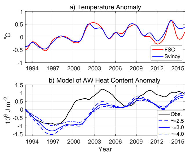
Figure 6. a) Sea surface EN4 temperature anomaly [ ^{\circ}\text{C} ] in the Faroe–Shetland Channel (FSC, red) and in the Svinøy Section (Svinoy, blue), used as proxies for the inflow temperature anomaly T'_i(t) . b) Modelled AW heat content anomaly (blue), which is obtained by integrating Eq. (14) forward in time, using the Svinøy Section temperatures and the e-folding timescales ( \tau ) equal to 2.5, 3.0, and 4.0 years. The black line shows the heat content AW anomaly estimated from the EN4 data; same data shown in Fig. 4 but here low passed with a 24 month running mean.
