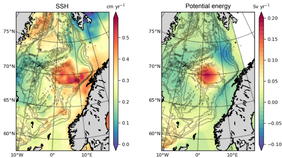
Figure 2. Left panel: Linear trend in SSH [cm yr -1 ] over the full altimetry period 1993-2017. Right panel: Linear trend in potential energy [Sv yr -1 ] (see Eq. (2)) from 1993-2016. Gray contours are bathymetry (Becker et al., 2009).
