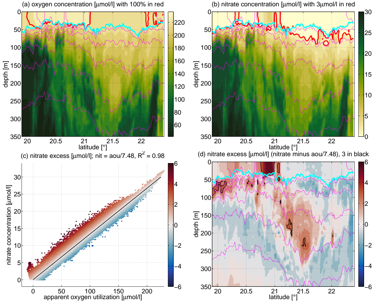
Figure 7. Sections of (a) oxygen concentration [μmol/l], (b) nitrate concentration [μmol/l], and (d) nitrate excess [μmol/l]. The following contours are highlighted: (a) 100% oxygen in red, (b) 3 μmol/l nitrate in red, and (d) 3 μmol/l nitrate excess in black. (c) all data in scatter plot of apparent oxygen utilization versus nitrate concentration where the black line is a best fit linear regression \text{nitrate} = \text{AOU}/7.48 . A nitrate excess of zero is on the black line in (c); positive/negative nitrate excess is colored red/blue above/below the black line in (c).
