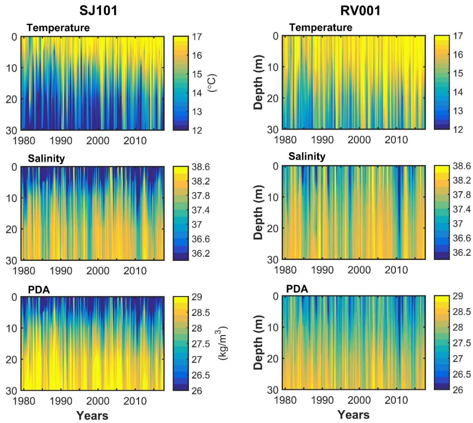
Figure 7. Hovmöller plots of temperature, salinity and PDA at SJ101 and RV001. Seasonal cycle has been removed.
