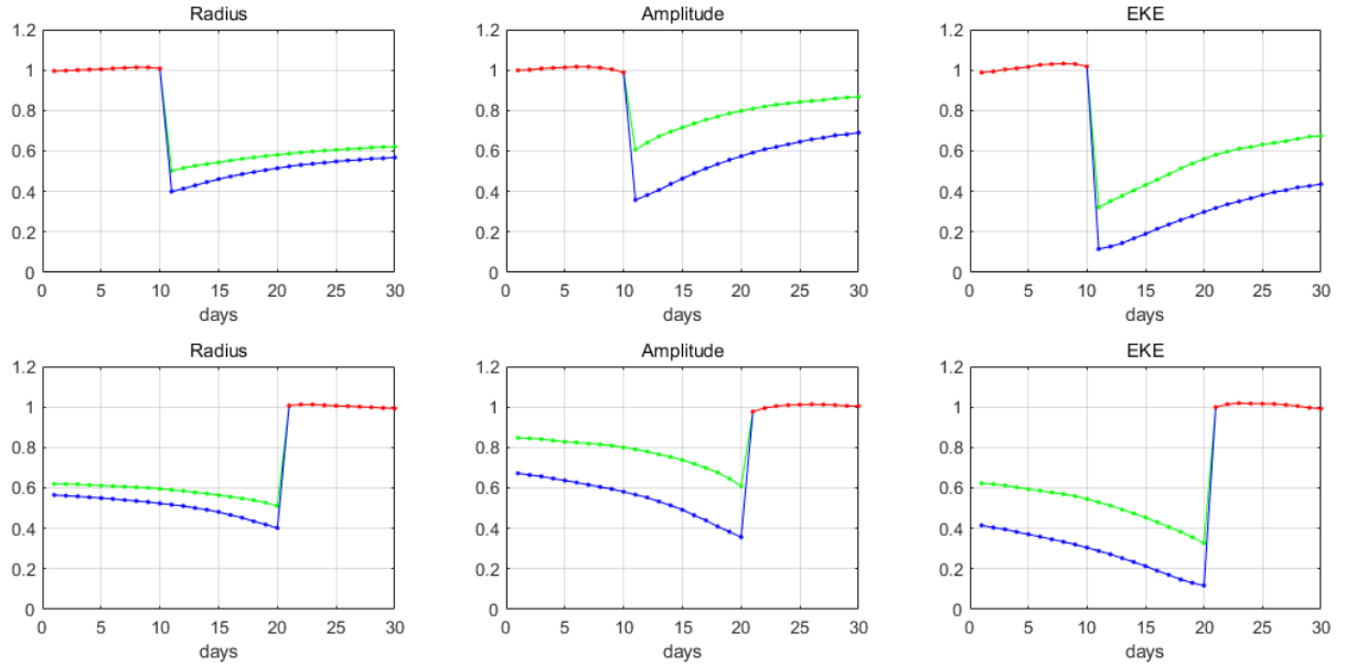
Figure 10. Average changes of eddy properties for all splitting (upper) and merging (lower) events. Properties of multicore eddies (red line) over 10 days and of single-core eddies (green and blue lines) over 20 days are presented. Properties of single-core eddies were normalized with respect to the multicore eddies.
