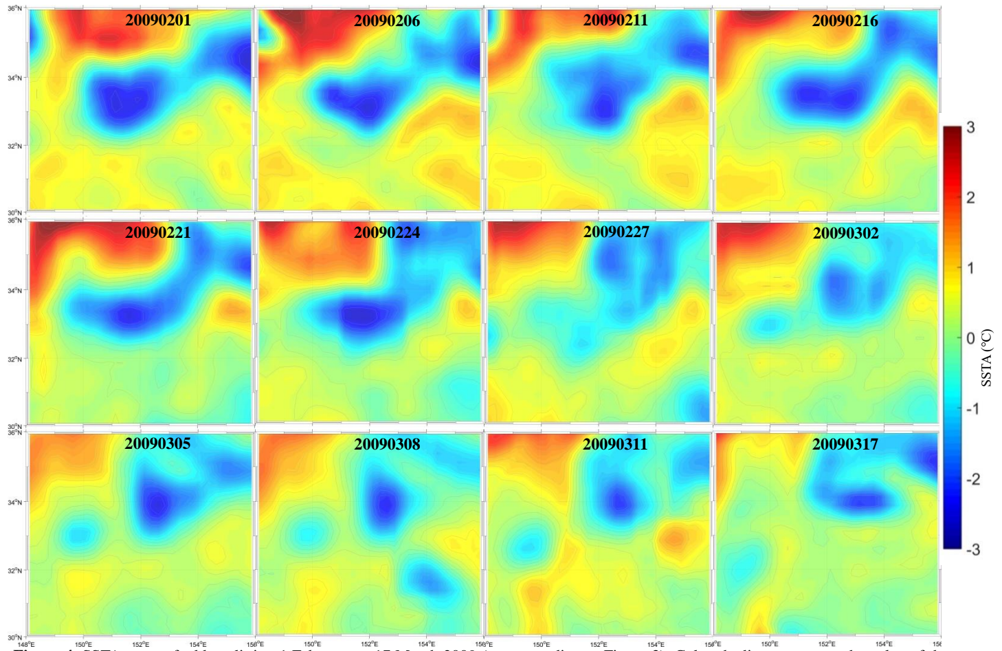
Figure 4. SSTA maps of eddy splitting 1 February to 17 March 2009 (corresponding to Figure 3). Color shading represents the value of the SSTA field.
