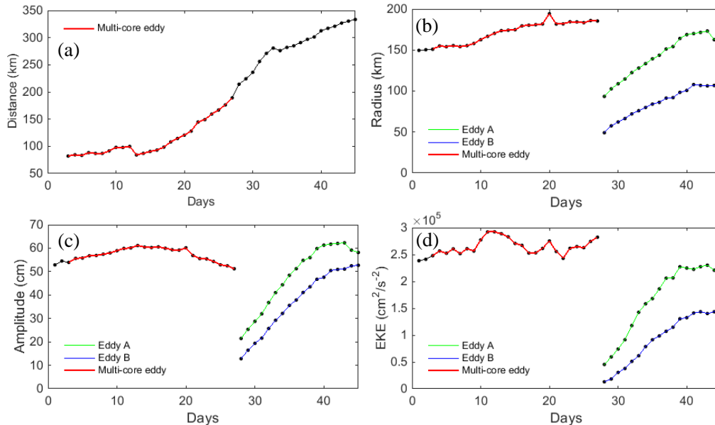
Figure 5. Changes of eddy properties with eddy split from 1 February to 17 March 2009: (a) distance between the two cores or two single eddies, (b) eddy scale, (c) eddy amplitude, and (d) eddy EKE. X axis represents the number of days from 1 February. The multicore eddy existed for 25 days from day 3 (3 February) to day 27 (27 February) and it split into two eddies on day 28 (28 February).
