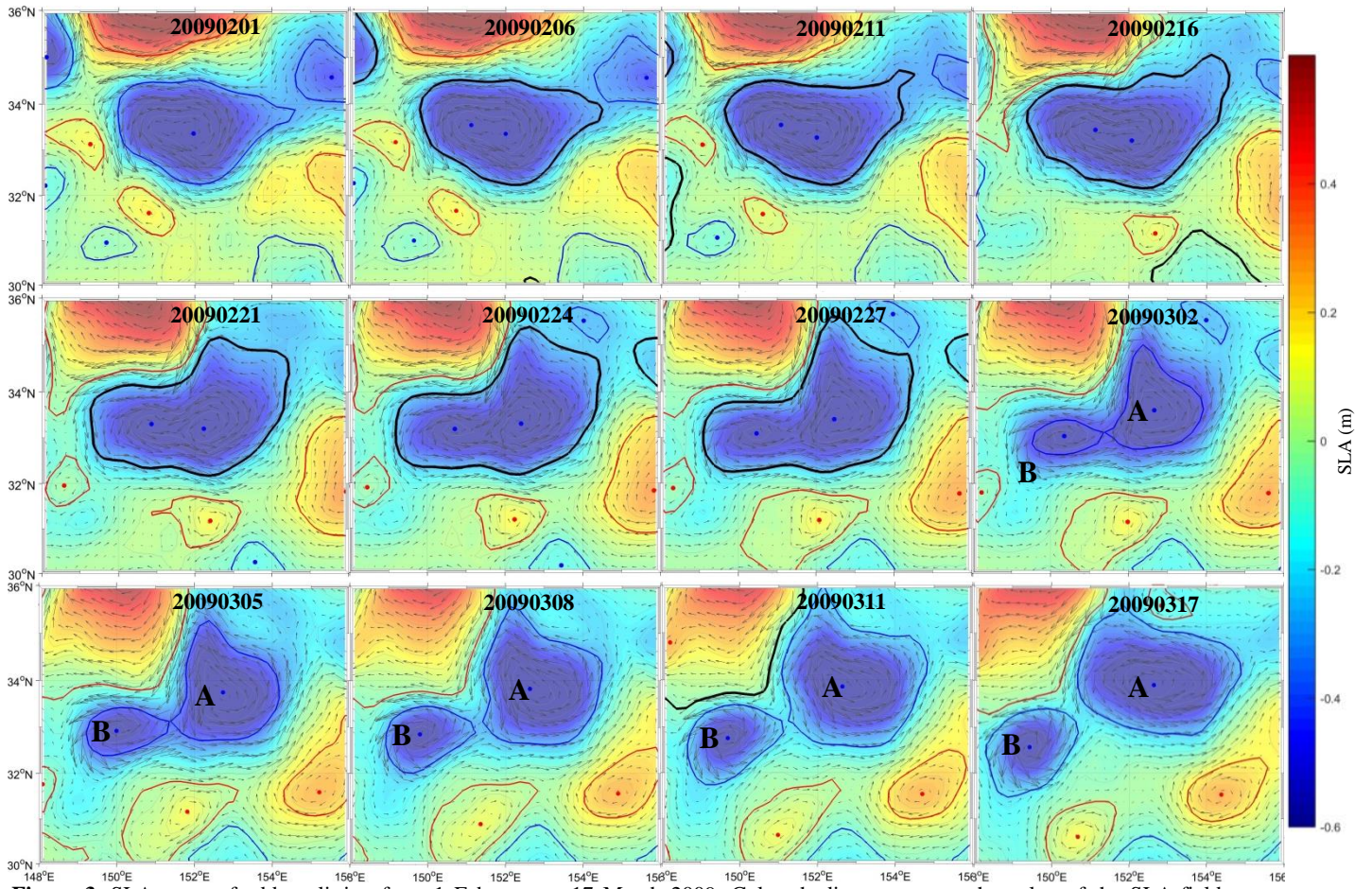
Figure 3. SLA maps of eddy splitting from 1 February to 17 March 2009. Color shading represents the value of the SLA field; arrows represent the surface geostrophic velocity components calculated from the SLA; blue and red lines represent boundaries of cyclonic and anticyclonic eddies, respectively; blue and red dots represent cyclonic and anticyclonic eddy cores, respectively; and black lines represent multicore eddies. For better observing the evolution process, the time interval between two adjacent maps is not the same, in the first row it is 5 days, the last map is after 6 days, and the other intervals are 3 days. The multicore eddy structure persisted for nearly a month before splitting.
