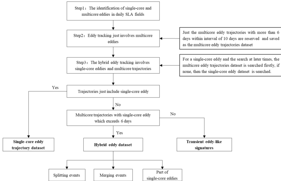
Figure 2. Flowchart of the eddy tracking process.
