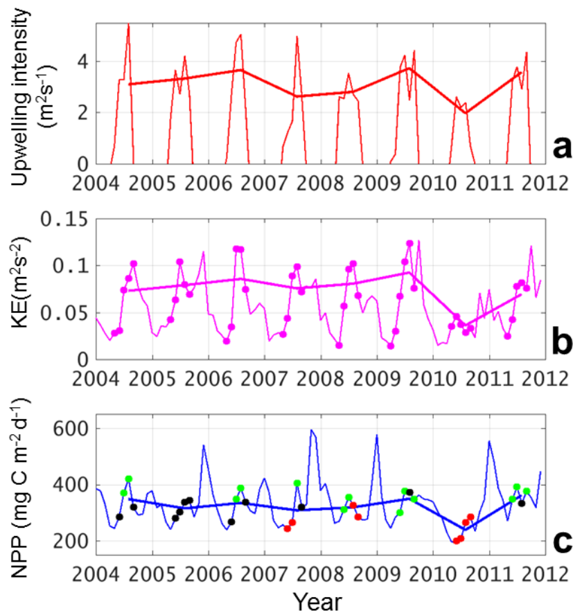
610 Figure 3 Time series of (a) UI in \text{m}^2 \text{s}^{-1} , (b) KE in \text{m}^2 \text{s}^{-2} and (c) NPP in \text{mg C m}^{-2} \text{d}^{-1} of monthly data (thin lines) and summer mean (thick lines). In (a), only the positive (upwelling-favorable) values are shown. In (b), months with positive UI are marked with dots. In (c), green, black and red dots indicate HNA, normal and LNA scenarios (see text for definition).
