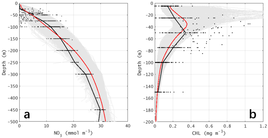
630 Figure 7 The vertical profiles of (a) nitrate concentration (unit: \text{mmol m}^{-3} ) and (b) chlorophyll concentration (unit: \text{mg m}^{-3} ). In both plots, the black dots are the observation values (see Fig. 1b for stations). The gray area are the envelop for all model stations in the same area and month, while the red lines are the area-mean profiles.
