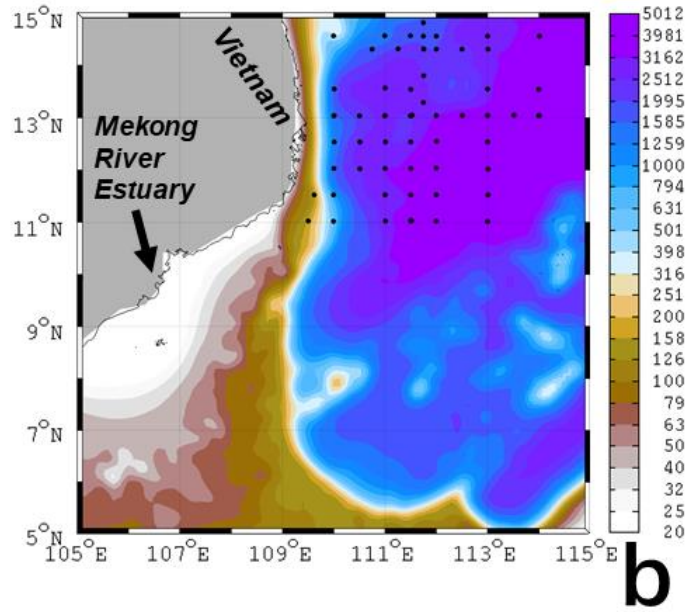
Figure 1 (a) Model domain and the bathymetry (unit: meter) for the TFOR-CoSINE model. Model grid nodes are shown every 25 points. The study area VBUS is boxed. (b) Zoom-in area of VBUS. Black diamonds are the observation stations (see text).
