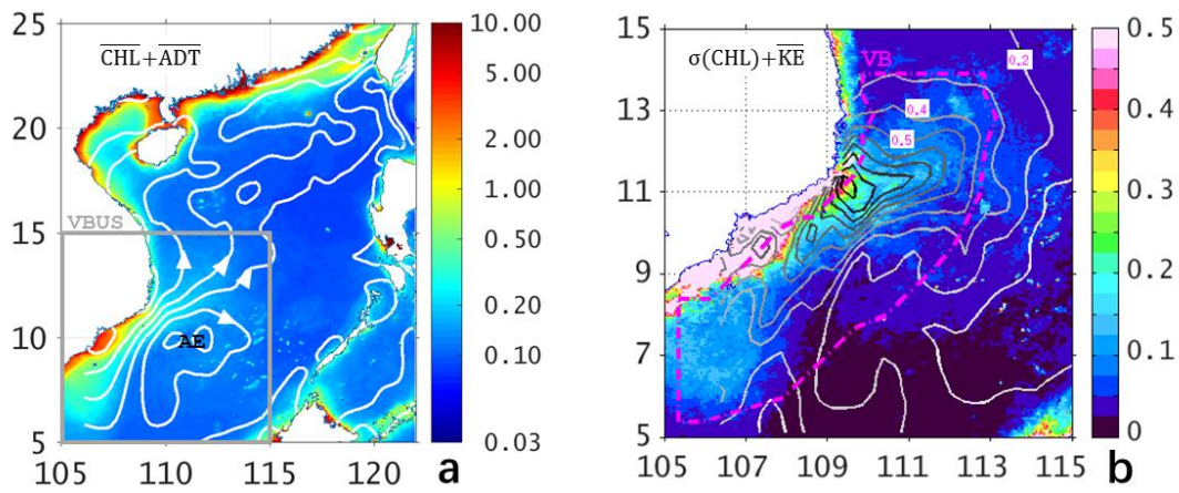
Figure 2 (a) Summertime (MJJAS) average of surface chlorophyll concentration (color shading, unit: \text{mg m}^{-3} ) from MODIS, overlapped white contours are mean ADT with the arrows showing the directions of surface currents. Gray box is the region of interest (VBUS), while AE shows the center of the anticyclone. (b) Standard deviation of surface chlorophyll (color shading, unit: \text{mg m}^{-3} ) overlapped with the contours of surface KE with an interval of 0.1 from 0.1 to 1.0 (unit: \text{m}^2 \text{s}^{-2} ). The magenta dot-dash contour delimits the ocean region over which chlorophyll and KE are averaged (see text).
