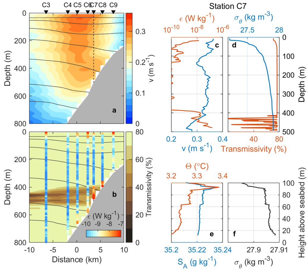
Figure 9. Distribution of a) the velocity component into the section and b) light transmissivity, together with selected isopycnals (black). Dissipation rate ( \log_{10}\epsilon ) is color coded in vertical columns in (b). Profiles collected at station C7: full depth profiles of c) dissipation rate and velocity and d) \sigma_\theta and transmissivity, and the bottom 100 m profiles of e) \Theta and S_A and f) \sigma_\theta .
