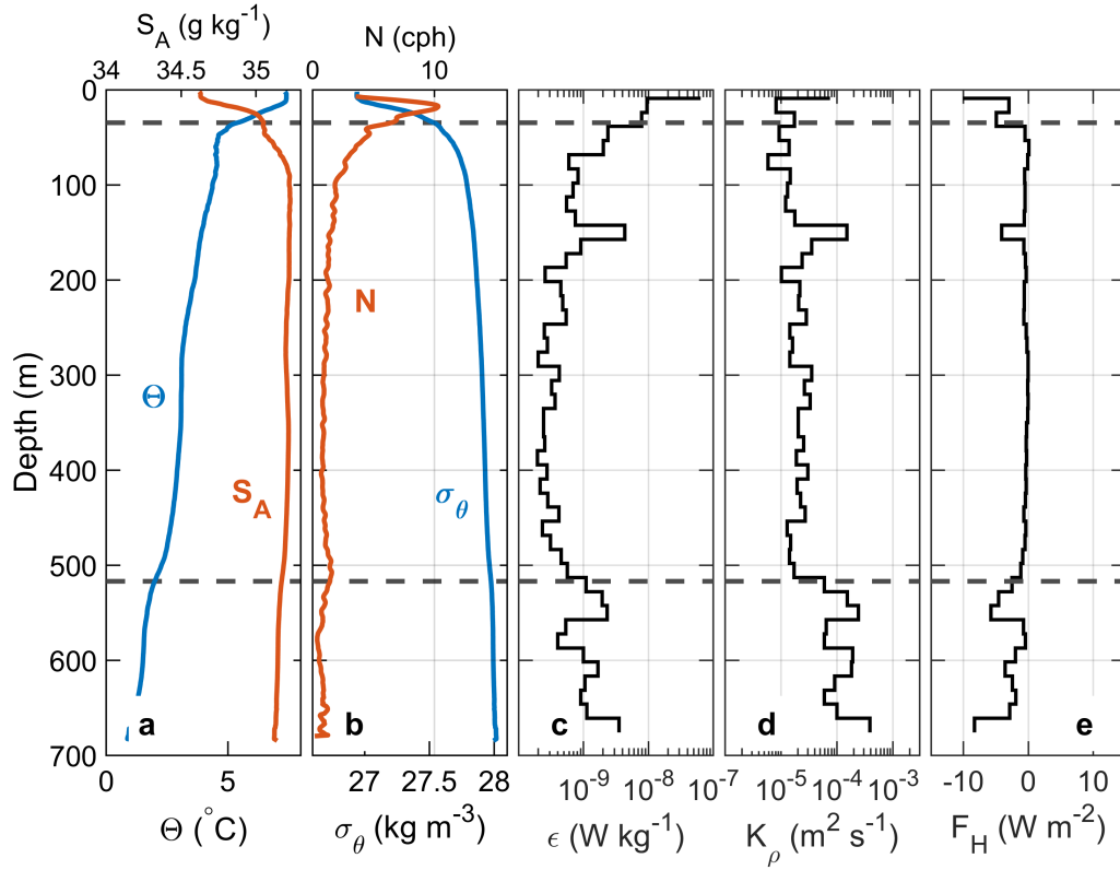
Figure 7. Temporal mean of measurements collected by the microstructure profiler at station R1, Section A. (a) \Theta (blue) and S_A (red), (b) \sigma_{\theta} (blue) and buoyancy frequency N (red), (c) 15-m bin-averaged dissipation of TKE \epsilon , (d) eddy diffusivity K_{\rho} , and (e) vertical heat flux F_H . Shaded bands envelop Dashed lines show the upper and lower boundaries of the stream tube. Water depth is 690 m.
