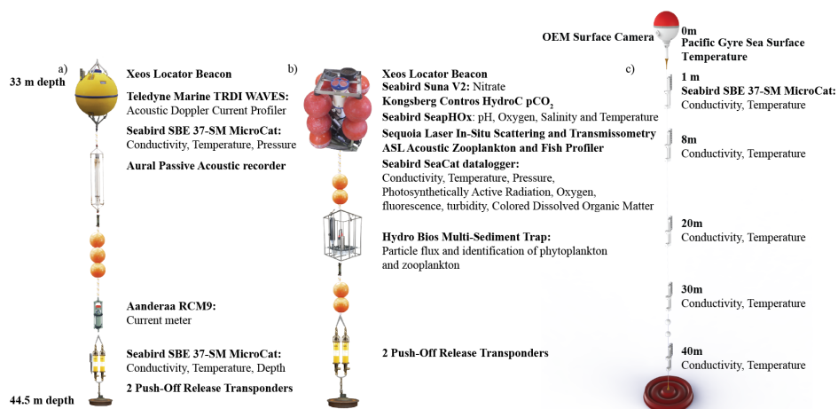
Figure 4: Illustration of the Chukchi Ecosystem Observatory (CEO), including the a) biophysical, b) biogeochemical, and c) freeze-up moorings. Note that the freeze up mooring includes a surface package, whereas the other two moorings only reach up to 33 m depth. Sensors are calibrated with as many in-situ samples as possible. Calibration samples are always collected upon deployment and recovery of the moorings, and depending on other research activity nearby our site, also at other times of the year. pCO 2 and pH sensors were added in summer 2016.
