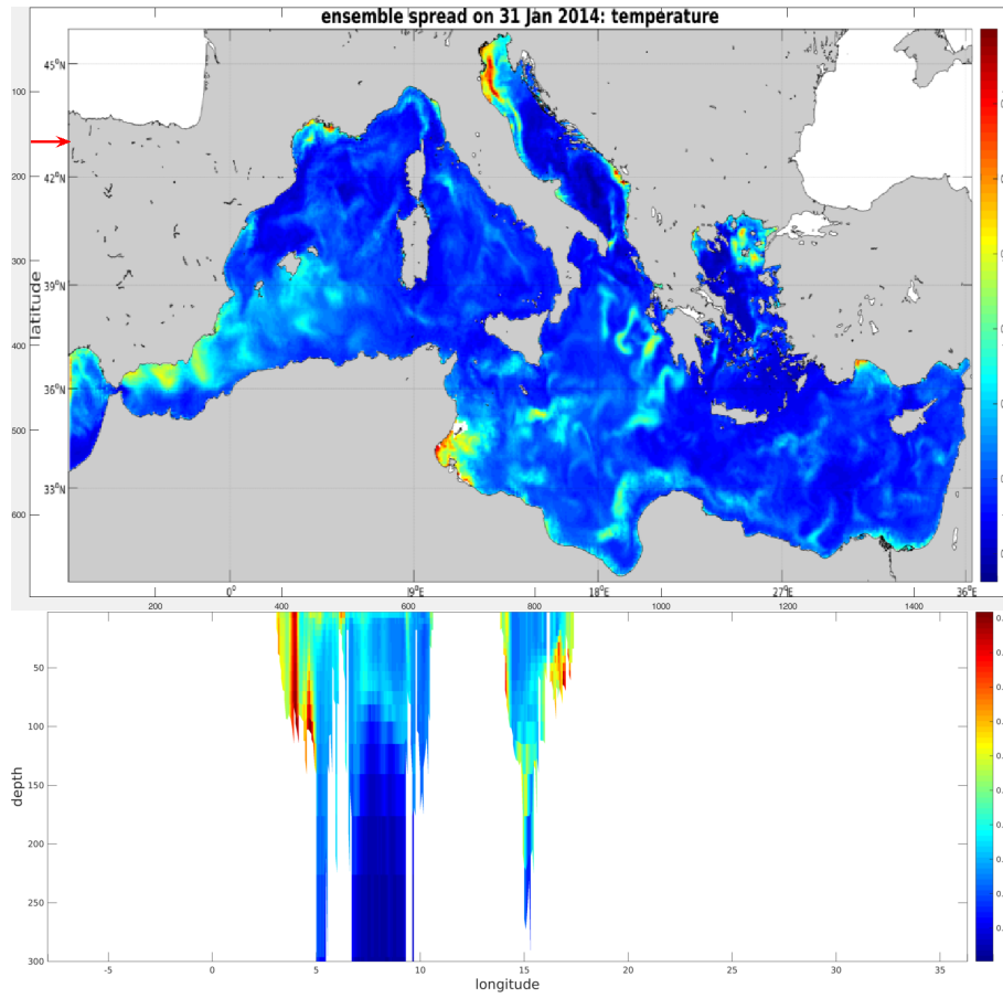
Figure 4. Spread of the ensemble of MED models at 31/01/2014: (upper panel) surface temperature, (lower panel) section at 43°N, indicated by a red arrow on the upper panel
