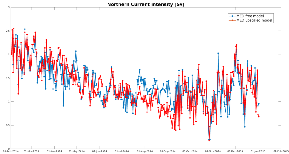
Figure 7. Water transport by the Northern current off Nice (France) during 2014, as obtained by the free (blue curve) and upscaled (red curve) parent models.
