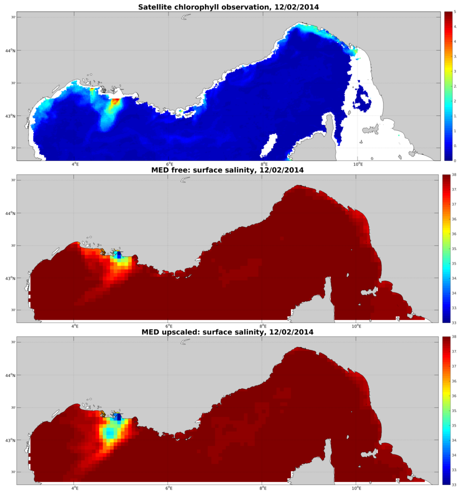
Figure 9. Comparison of the Rhône river plume on 12/Feb/2014 (upper panel) satellite chlorophyll image (middle panel) free parent model salinity (lower panel) and upscaled parent model salinity
