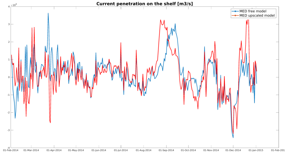
Figure 6. Water transport across the shelf break during 2014, as obtained by the free (blue curve) and upscaled (red curve) parent models. Positive values indicate a net on-shelf transport.
