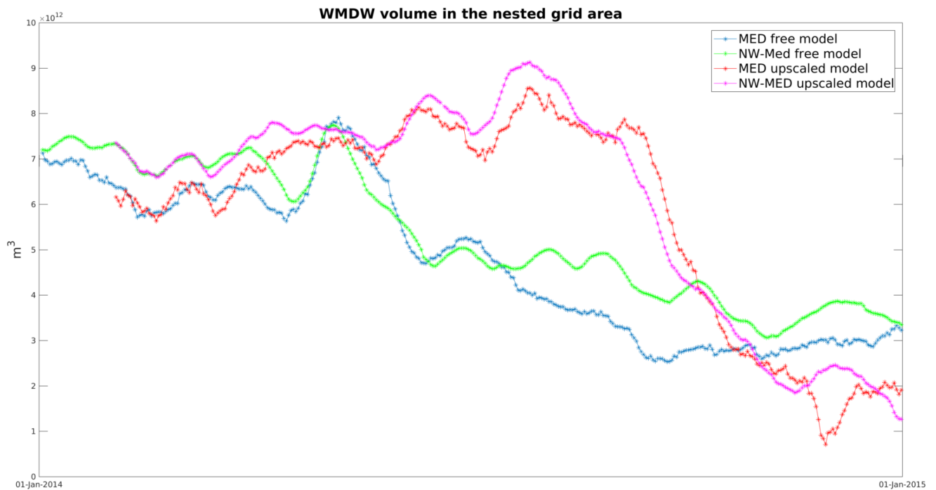
Figure 11. Time series of total amount of WMDW in the area covered by the nested model: (blue) free parent model (green) nested model in the free model (red) parent model with upscaling (magenta) nested model in the upscaled model
