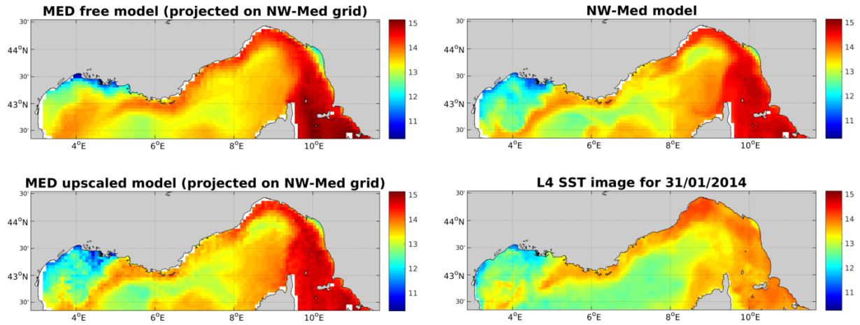
Figure 5. Sea surface temperature after the first upscaling step (31/01/2014), in the free model (upper left), nested model (upper right), upscaled model (lower left) and L4 satellite observation (lower right)
