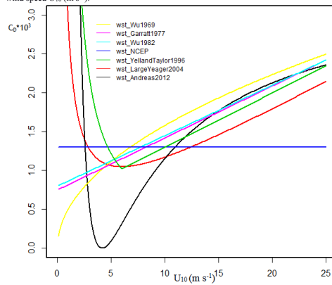
Figure 1. The drag coefficient parameterization used in the study (Eqs. 7-13) as a function of wind speed U_{10} ( \text{m s}^{-1} ).
