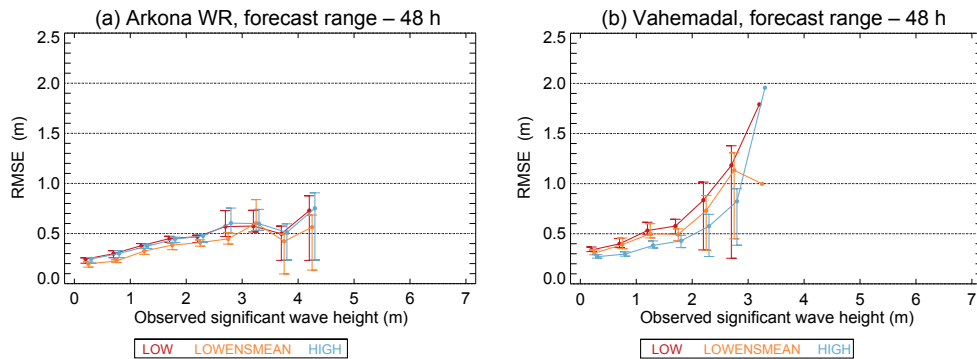
Figure 8. RMSE as function of SWH for the Arkona WR (a) and Vahemadal sites (b) for the LOW, LOWENSMEAN and HIGH forecasts with a forecast range of 48 h. Error bars show the 5 % and 95 % confidence bands calculated by bootstrapping.
