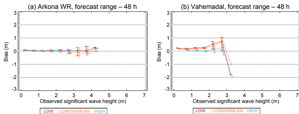
Figure 9. Bias as function of SWH for the Arkona WR (a) and Vahemadal sites (b) for the LOW, LOWENSMEAN and HIGH forecasts with a forecast range of 48 h. Error bars show the 5 % and 95 % confidence bands calculated by bootstrapping.
