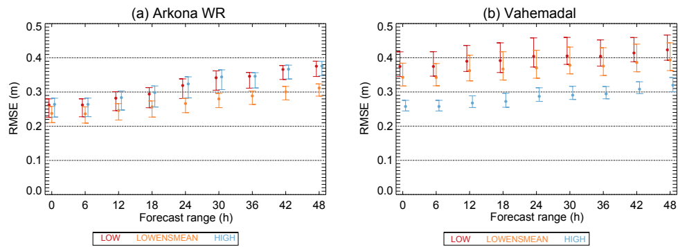
Figure 7. RMSE for selected forecast ranges for the Arkona WR (a) and Vahemadal site (b) for the LOW, LOWENSMEAN and HIGH forecasts. Error bars show the 5 % and 95 % confidence bands calculated by bootstrapping.
