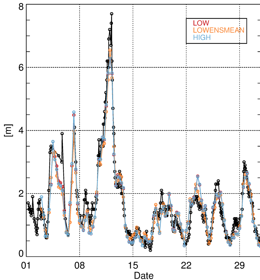
Fig. 2. Observed and forecasted (48 hour) SWH for Northern Baltic during storm Toni
