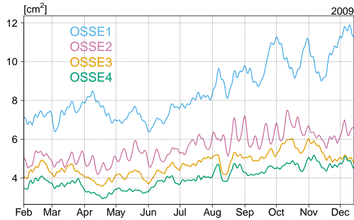
Figure 4. Temporal evolution of the SSH error variance in the ocean analysis over the period February-December 2009. Results obtained comparing the SSH of the ocean analysis in the experiments OSSE1 (blue line ) and OSSE2 (purple line), OSSE3 ( red-orange line) and OSSE4 (green line) with the data of the NR considering the ocean areas with a bathymetry deeper than 200 metres; y-axes expressed as [cm^2] . OSSE0 (not shown) ranged between 25 and 35 cm^2 .
