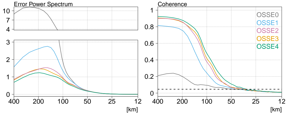
Figure 7. Spectral Analysis of the SSH signals in the OSSEs considering an open ocean region (-19°W, -10°W; 46.N, 55°N) representative of the North Atlantic Drift, during the period February-December 2009. In the panels the The results for the experiments OSSE0 (gray lines), OSSE1 (blue lines), OSSE2 (purple lines), OSSE3 (red-orange lines) and OSSE4 (green lines), are shown at the spectral window between 400 km and 12 km. Left panel: power spectra of the SSH error, with respect to the NR; the spectra are shown in a variance preserving form [ cm^2 ]. Right panel: spectral coherence in the OSSEs with respect to the NR; black dashed line shows the 95 % confidence interval (Thomson and Emery, 2014).
