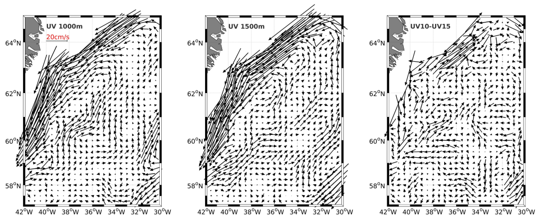
Fig. 1. Irminger Sea circulation in depth layers
