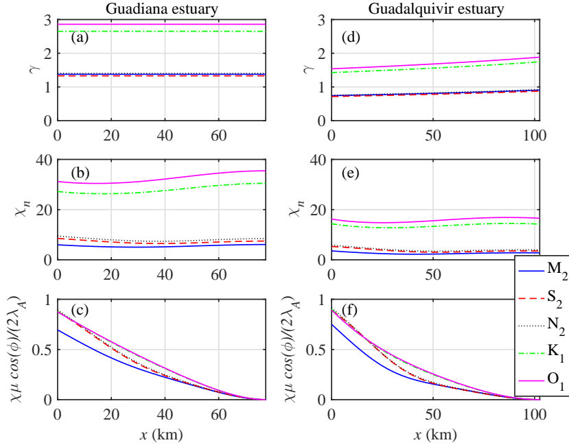
Figure 10. Longitudinal variations of estuary shape number \gamma (a, d), friction number \chi_n (b, e) and \chi_n \mu \cos(\phi)/(2\lambda_A) (c, f) in the Guadiana estuary (a, b, c) and Guadalquivir estuary (d, e, f).
