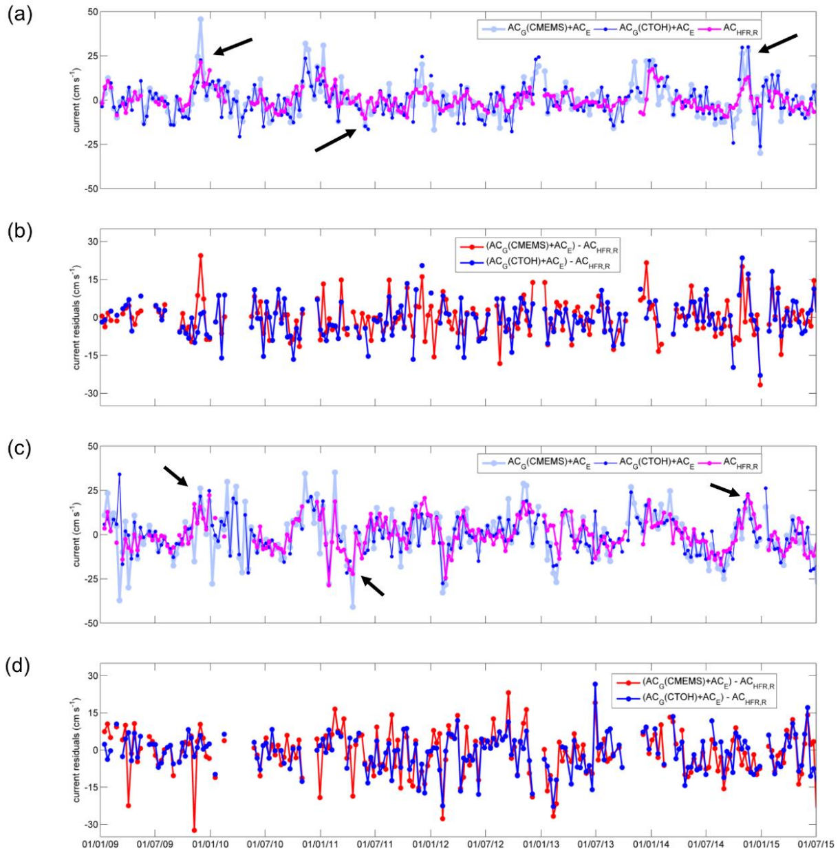
Figure 3. Across-track AC_G+AC_E and AC_{\text{HFR,R}} . (a) CTOH, CMEMS and HFR data sets in point ER. (b) CTOH-HFR and CMEMS-HFR residuals in point ER. (c) CTOH, CMEMS and HFR data sets in point WR. (d) CTOH-HFR and CMEMS-HFR residuals in point WR. Black arrows depict the slope current intensifications mentioned in the text.
