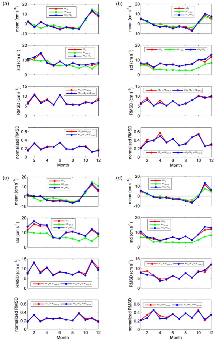
Figure 4. Monthly statistical parameters of the comparison between AC_G vs AC_{HFR,R} and AC_G + AC_E vs AC_{HFR,R} in the points E_R and W_R for both altimetry products: (a) CTOH AC_G in point W_R , (b) CTOH AC_G in point E_R , (c) CMEMS AC_G in point W_R , (d) CMEMS AC_G in point E_R . The normalized RMSD is the quotient between the RMSD and the values of the corresponding AC_{HFR,R} .
