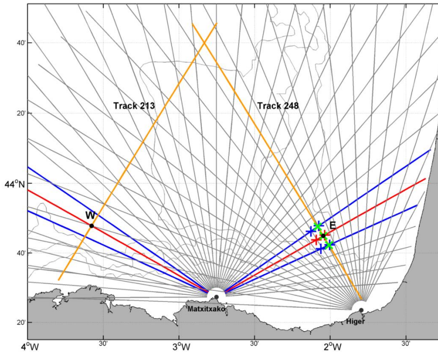
5 Figure 2. Schematic view of the pointwise comparison and of the data used for this approximation. Jason-2's 213 and 248 tracks are depicted by orange lines. The HFR radial directions from both sites are represented by grey lines and the selected radial directions (from Matxitxako site) for the pointwise comparison are plotted in red (i.e. the central radial orthogonal to the track) and in blue (the adjacent radials). Points E and W are those along both tracks, where each of the HFR radial directions are orthogonal to the Jason-2's tracks directions. At point E, the blue and red crosses show the selected points of HFR radial directions where radial currents are averaged in a first step to obtain the 10 corresponding values on the track (green crosses). Then, the along-track green crosses are averaged to obtain the corresponding HFR current values in the point at issue (the same process is carried out for point W, but it is not represented in the figure). Grey lines: 200, 1000, and 2000 m isobaths.
