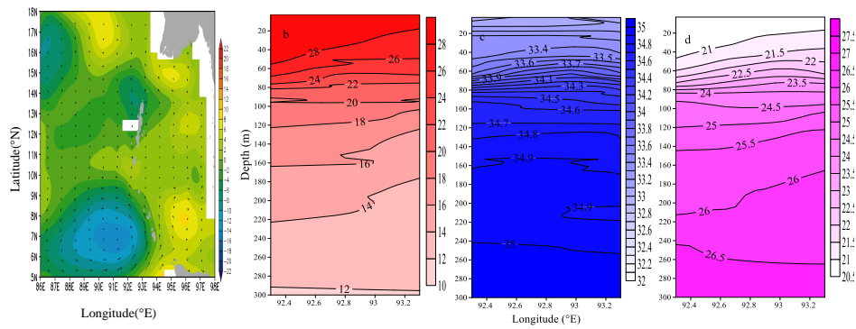
Fig. 2 a) Sea Surface Height (cm- Aviso weekly) and geostrophic current (cm/s) and the eddy location b) Vertical temperature ( ^{\circ}\text{C} ), c) salinity and d) density ( \text{kg}/\text{m}^3 ) distribution at the eddy location
