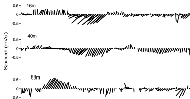
Fig. 3 Horizontal current (m/s) structure at different depth at 8^{\circ}\text{N}
