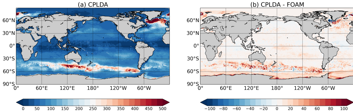
Figure 8. Annual mean Kara mixed layer depth in m (Kara et al. (2000) using temperature criterion of 0.8^{\circ}\text{C} : (a) CPLDA, and (b) difference between CPLDA and FOAM. Positive value means CPLDA MLD is deeper than FOAM MLD.
