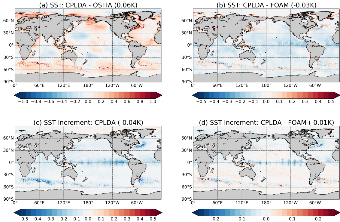
Figure 6. CPLDA SSTs in 2015 compared to (a) OSTIA (0.06 K) and (b) FOAM (-0.03 K); (c) mean SST increments in 2015 for CPLDA (-0.04 K); (d) mean SST increments in 2015 for CPLDA compared to FOAM (-0.01 K). Values in parentheses are averages for the global ocean.
