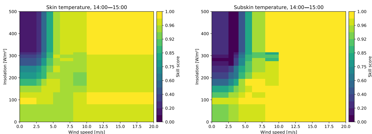
Figure 5. Skill score of the CCA OO compared to the parameterisation of Bernie et al. (2007).
