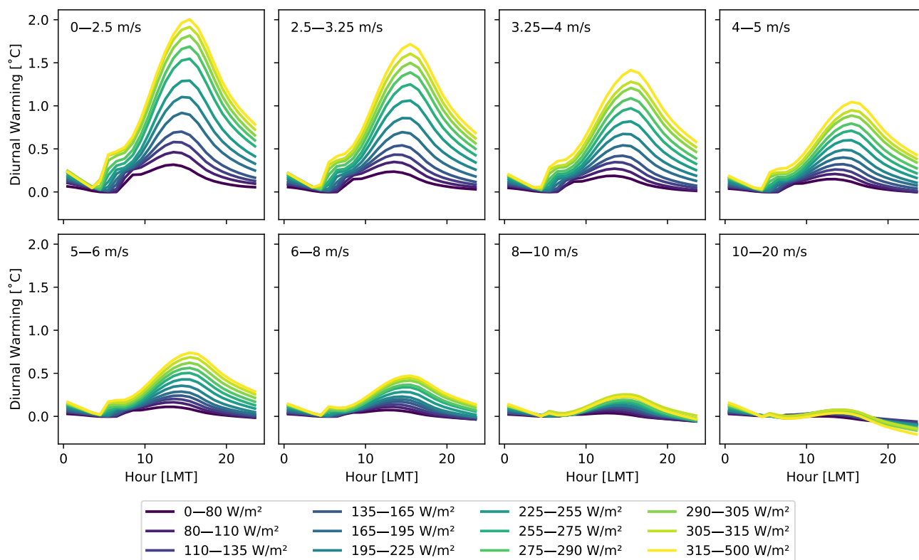
Figure 1. The magnitude of the diurnal warming as a function of the time of the day for different wind and insolation categories. The diurnal warming is measured with respect to the SST at local sunrise. The wind categories are represented by the different panels, while the insolation categories are shown as different curves within each panel.
