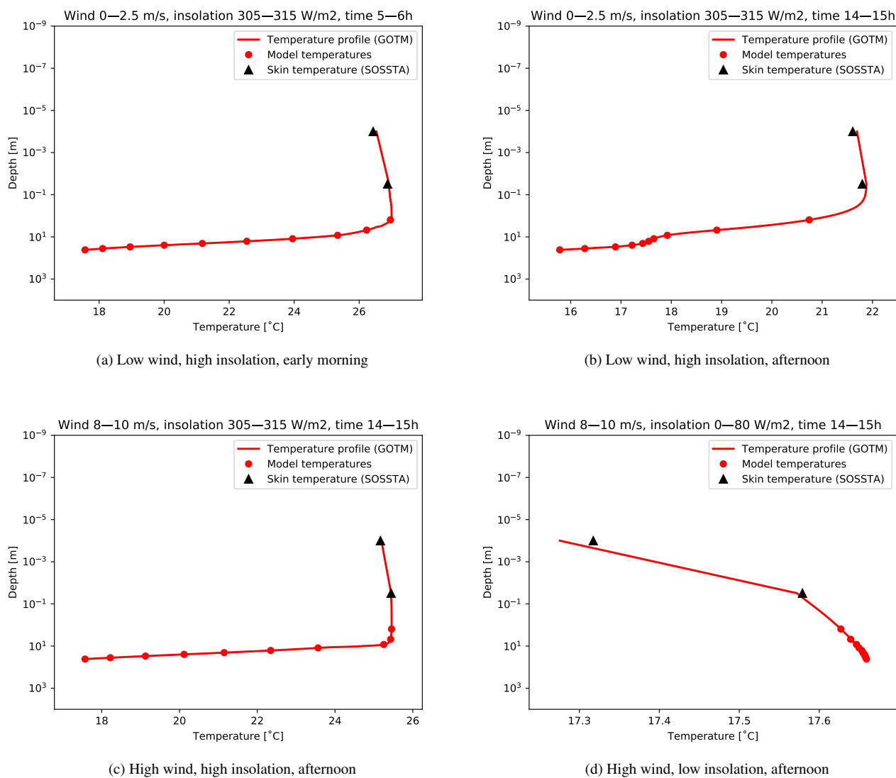
Figure 3. Examples of temperature profiles in various conditions and at different times. The GOTM profiles are shown by the red curve, while the red dots indicate the values used as input to the CCA OO. The output of the CCA OO is shown by the black triangles.
