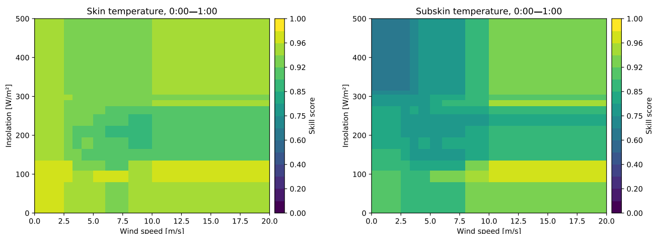
Figure 4. Skill score of the CCA OO compared to upper model level for all wind and insolation categories at midnight.
