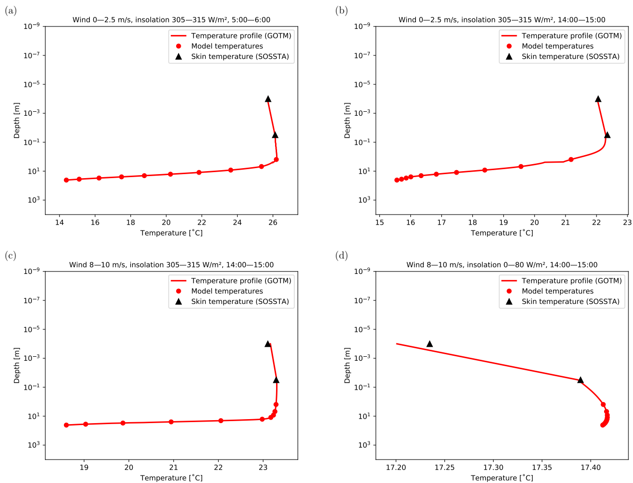
Figure 3. Examples of temperature profiles in various conditions and at different times. The GOTM profiles are shown by the red curve, while the filled circles indicate the values used as input to the CCA OO. The output of the CCA OO is shown by the black triangles. (a) Low wind, high insolation, early morning; (b) Low wind, high insolation, afternoon; (c) High wind, high insolation, afternoon; (d) High wind, low insolation, afternoon.
