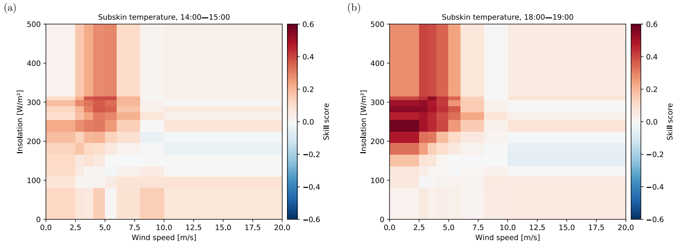
Figure 5. Skill score of the CCA OO compared to the parameterisation of Bernie et al. (2007) in the afternoon (a) and early evening (b).
