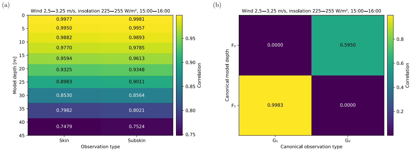
Figure 2. The correlation coefficients between the model variables and observations (a); and the canonical equivalent of these variables (b).
