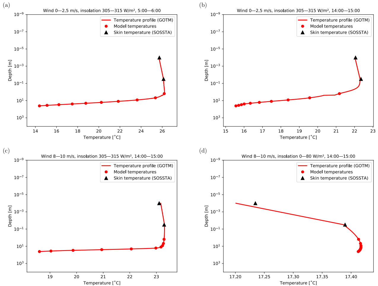
Figure 3. Examples of temperature profiles in various conditions and at different times. The GOTM profiles are shown by the red curve, while the filled circles indicate the values used as input to the CCA OO. The output of the CCA OO is shown by the black triangles. (a) Low wind, high insolation, early morning; (b) Low wind, high insolation, afternoon; (c) High wind, high insolation, afternoon; (d) High wind, low insolation, afternoon.
