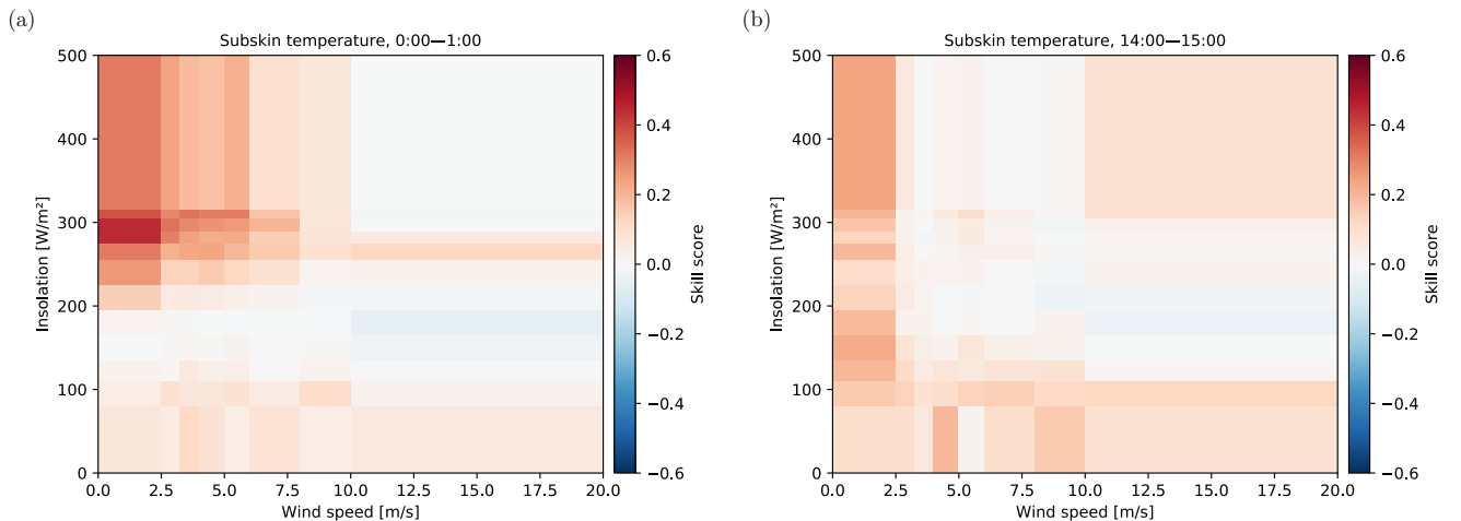
Figure 4. Skill score of the CCA OO compared to the OGCM upper layer for all wind and insolation categories at midnight (a) and in the afternoon (b).
