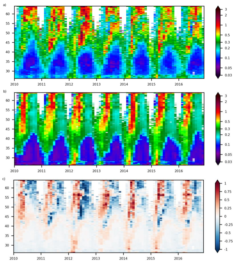
Figure 3. Hovmöller diagram for sea surface Chl-a at 15°W between 2010 and 2016. a) ESA OC-CCI ocean colour product, 950 b) IBI36 and c) bias of Chl-a ( model - obs ), all expressed in mg Chl m -3 . Monthly fields between 2010 and 2016 are used.
