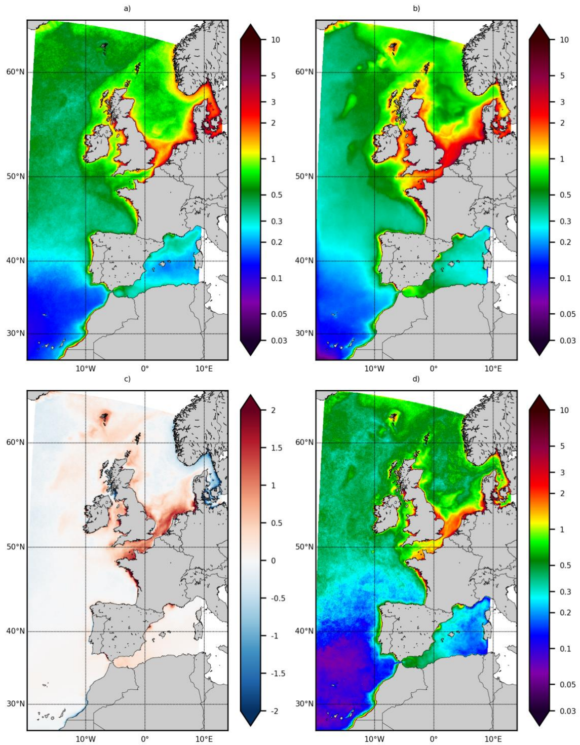
Figure 2. Sea surface Chl-a. a) annual average of ESA OC-CCI ocean colour product, b) annual average of IBI36, c) averaged bias of Chl-a ( model - obs ) and and d) RMSE ( \sqrt{\langle (model - obs)^2 \rangle} ), all expressed in mg Chl m -3 . Statistics are computed from monthly fields between 2010 and 2016.
