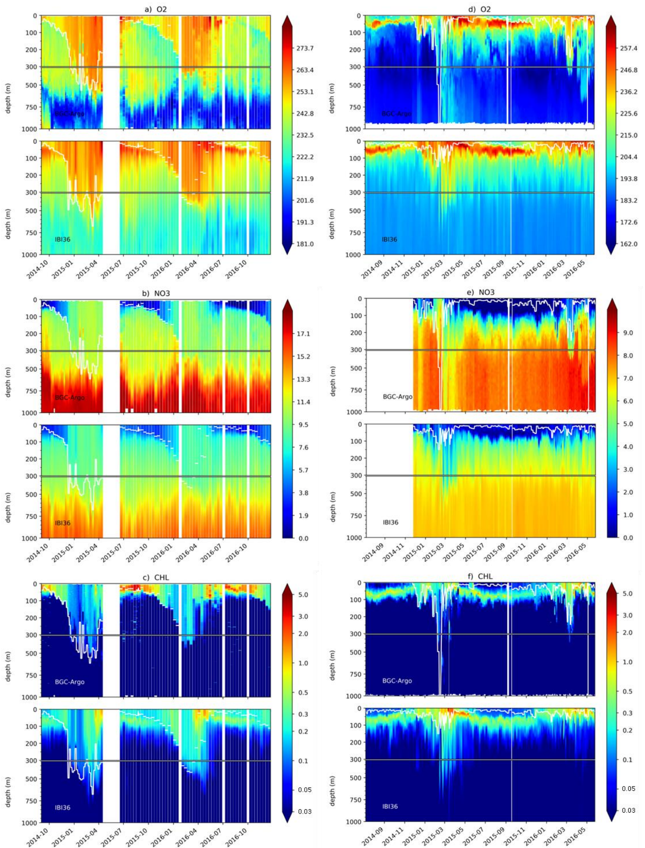
1060 Figure 16. Time series of oxygen (top), nitrate (middle), and Chl-a (bottom) from BGC-Argo data and IBI36 for the Atlantic (left) and Mediterranean (right). Oxygen and nitrate are expressed in \mu\text{mol l}^{-1} and Chl-a in \text{mg Chl m}^{-3} . IBI36 and Argo data are collocated in space and time. The white line represents the MLD computed from density criterion of 0.03 \text{ kg m}^{-3} difference from surface.
