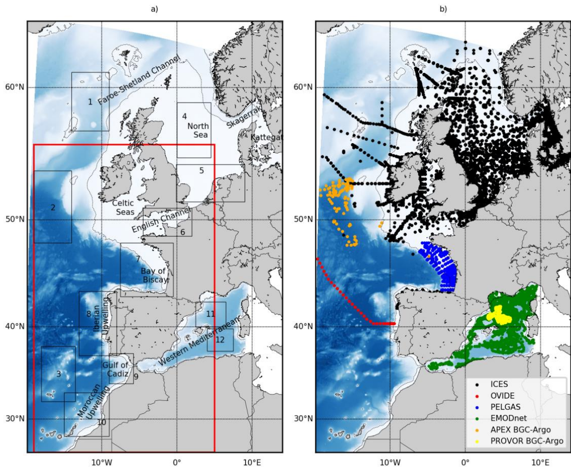
Figure 1. a) IBI Extended Domain on a curvilinear grid and IBI Service Domain extending from -19^{\circ}\text{E} to 5^{\circ}\text{E} and 26^{\circ}\text{N} to 56^{\circ}\text{N} on a regular grid (red rectangle). The 12 back boxes represent the different areas described in Section 2 and used for evaluation in Section 4. They represent the North Atlantic (boxes 1, 2, 3), North Sea (boxes 4 and 5), English Channel (box 6), Bay of Biscay (box 7), Iberian upwelling (box 8), Gulf of Cadiz (box 9), Moroccan upwelling (box 10) and Western Mediterranean (boxes 11 and 12). b) Location of in-situ biogeochemical data used for validation. ICES data are in black, OVIDE section and PELGAS data of the North-East Atlantic EMODnet dataset are respectively in red and blue, the Mediterranean Sea EMODnet dataset is in green, the APEX BGC-Argo float in the Atlantic is in orange, and PROVOR BGC-Argo float in the Mediterranean is in yellow. The blue colour shading represents the bathymetry and dashed line is the 200 m isobath delimiting the shelf region.
