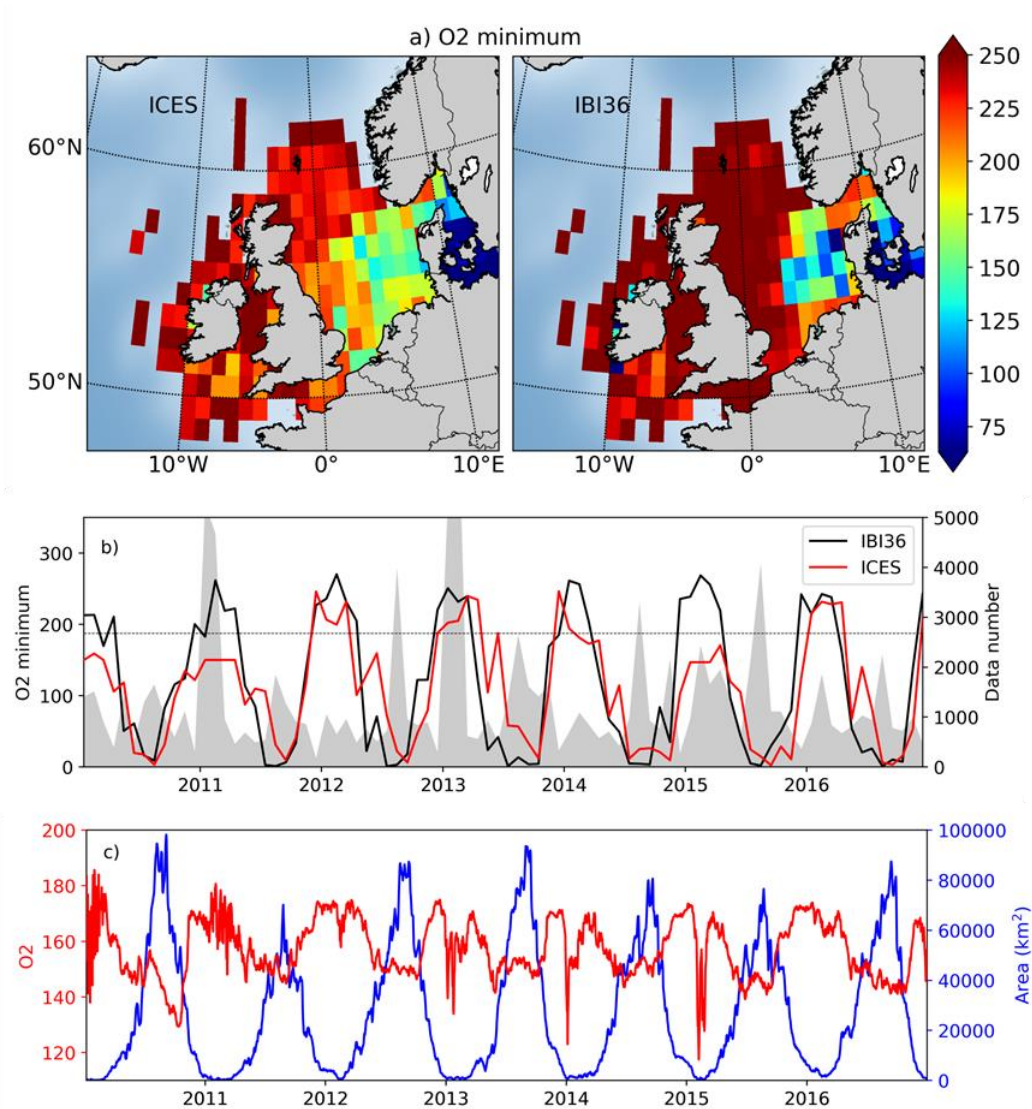
Figure 11: a) Minimum oxygen ( \mu\text{mol l}^{-1} ) in ICES data (left) and IBI36 collocated to ICES (right) between 2010 and 2016. 1020 b) Time series of minimum oxygen ( \mu\text{mol l}^{-1} ) in ICES data (red) and IBI36 IBI36 collocated to ICES (black). The deficiency 1025 threshold of oxygen ( 6 \text{ mg l}^{-1} or 187.5 \mu\text{mol l}^{-1} ) is represented by the dashed line. Number of available data in ICES is added to the right axis (area plot in gray). c) Surface area (in \text{km}^2 ) vulnerable to oxygen deficiency, that is where oxygen decrease below the deficiency threshold (blue; right axis) and associated mean oxygen concentrations ( \mu\text{mol l}^{-1} ; red; left axis) using the whole IBI36 simulation (not only IBI36 collocated to ICES). The three subplots are for the continental shelf (bathymetry \leq 200\text{m} ).
