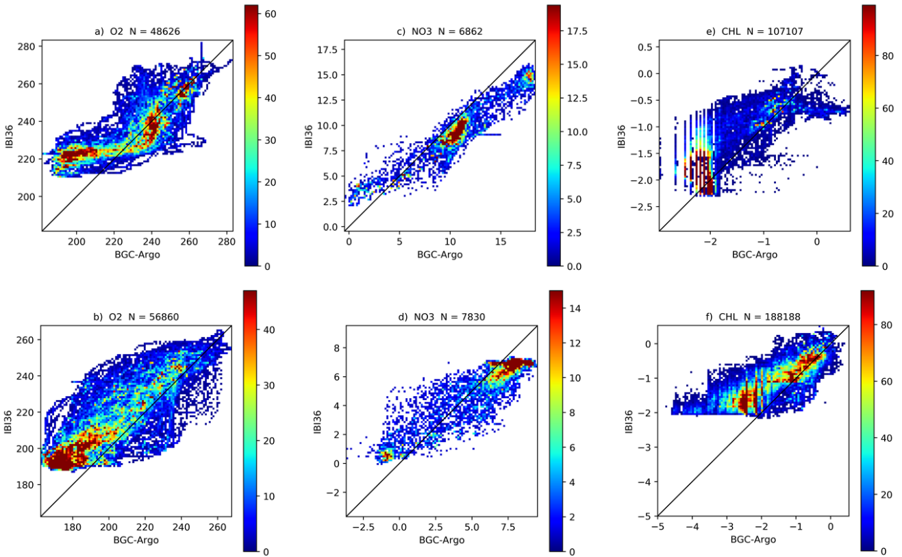
Figure 15. Density plots for oxygen (a, b), nitrate (c, d), and log(Chl-a) (e, f) from BGC-Argo data and IBI36 for the Atlantic (top) and Mediterranean (bottom). Oxygen and nitrate are expressed in \mu\text{mol l}^{-1} . Argo data are on the x-axis and IBI36 on the y-axis of the density plots. Each axis is divided in 100 bins and colorbar represents the density of the match-ups (number of overlapping points). Note the different scales for the variables. N indicates the total number of match-ups. IBI36 and Argo data are collocated in space and time.
