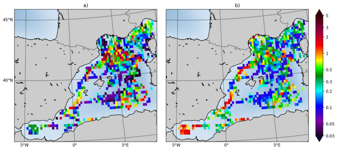
1045 Figure 14. Sea surface Chl-a from EMODnet dataset (a) and IBI36 (b) in mg Chl m -3 . IBI36 and EMODnet dataset are collocated in space and time between 2010 and 2016. Match-ups are averaged between 0 and 10 meter depth, gridded and averaged on a horizontal grid of 0.2°x0.2° resolution.
