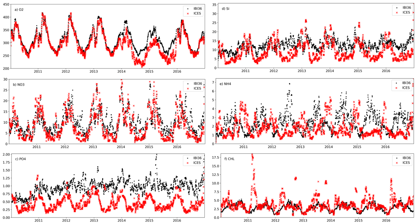
1010 Figure 10. Time series of surface concentrations of a) oxygen, b) nitrate, c) phosphate, d) silicate, e) ammonium and f) Chl-a from ICES (red) and IBI36 (black). Oxygen and nutrients are expressed in \mu\text{mol l}^{-1} and Chl-a in \text{mg Chl m}^{-3} . Daily averaged IBI36 outputs and ICES data are collocated in space and time between 2010 and 2016. Match-ups are averaged between 0 and 10 meter depth, and daily averaged. Time series are smoothed using a 10-day window.
