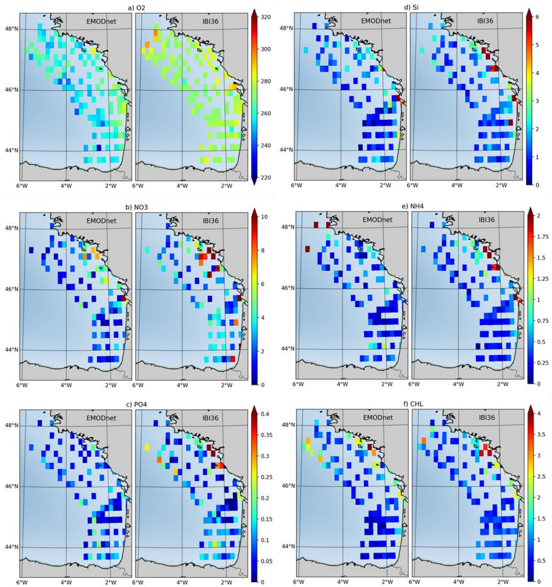
1040 Figure 13. Surface concentrations of oxygen (a), nitrate (b), phosphate (c), silicate (d), ammonium (e) and Chl-a (f) from the PELGAS data of the EMODnet database (left of each panel) and IBI36 (right of each panel). Oxygen and nutrients are expressed in \mu\text{mol l}^{-1} and Chl-a in \text{mg Chl m}^{-3} . IBI36 and PELGAS data are collocated in space and time between 2010 and 2016. Match-ups are averaged between 0 and 10 meter depth, gridded and averaged on a horizontal grid of 0.2^\circ \times 0.2^\circ resolution.
