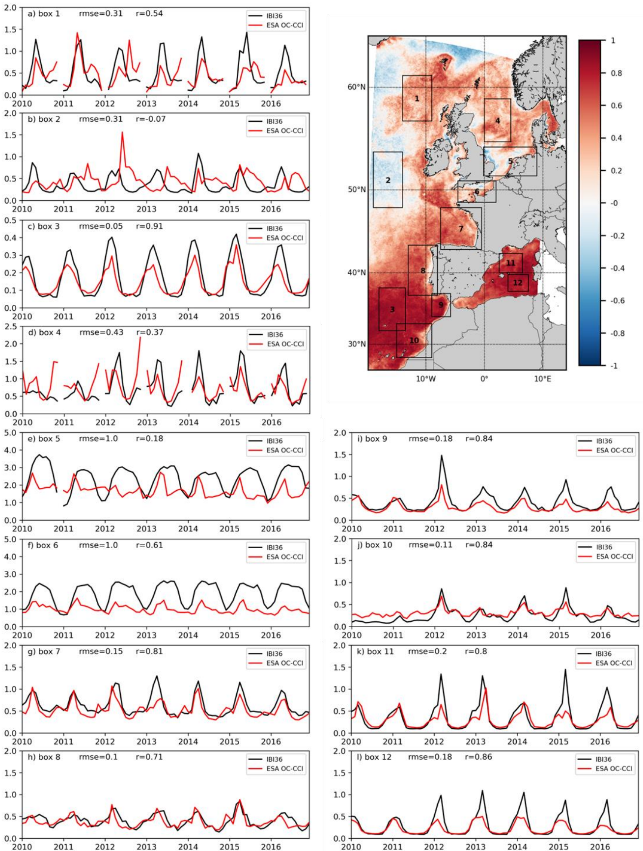
955 Figure 4. Time series of Sea surface Chl-a ( \text{mg Chl m}^{-3} ) between 2010 and 2016. IBI36 is in black and ESA OC-CCI ocean colour product in red. Chl-a is averaged over the 12 boxes defined in Figure 1 and reported to the map on the top-right. The RMSE ( \sqrt{\langle (model - obs)^2 \rangle} ) and correlation ( r ) between the model and the data are indicated for each time series. The top-right panel represents the spatial distribution of temporal correlation between the model and the observation. Note the different scales in y-axis.
