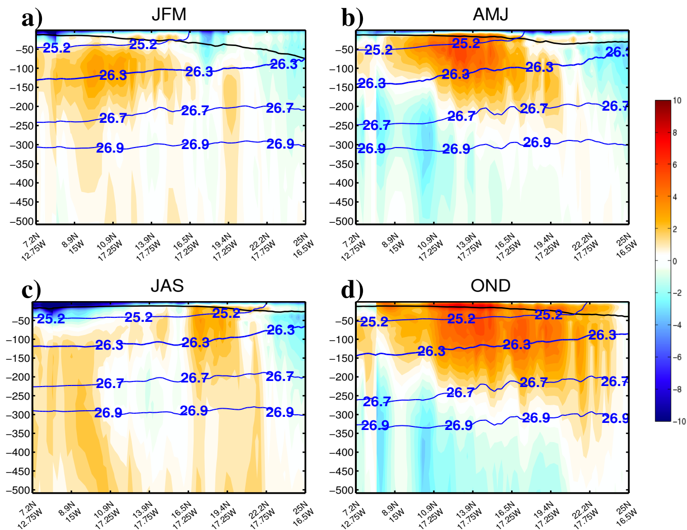
Figure 9. Seasonally averaged vertical section of along-slope velocity (in colors; [ \text{cm s}^{-1} ]), \sigma_t (blue lines; [ \text{kg m}^{-3} ]), and mixed layer depth (black line; [ \text{m} ]) following the shelf break (across-shore averaging between the 100m isobath and 6 grid points - 150 km - offshore).
