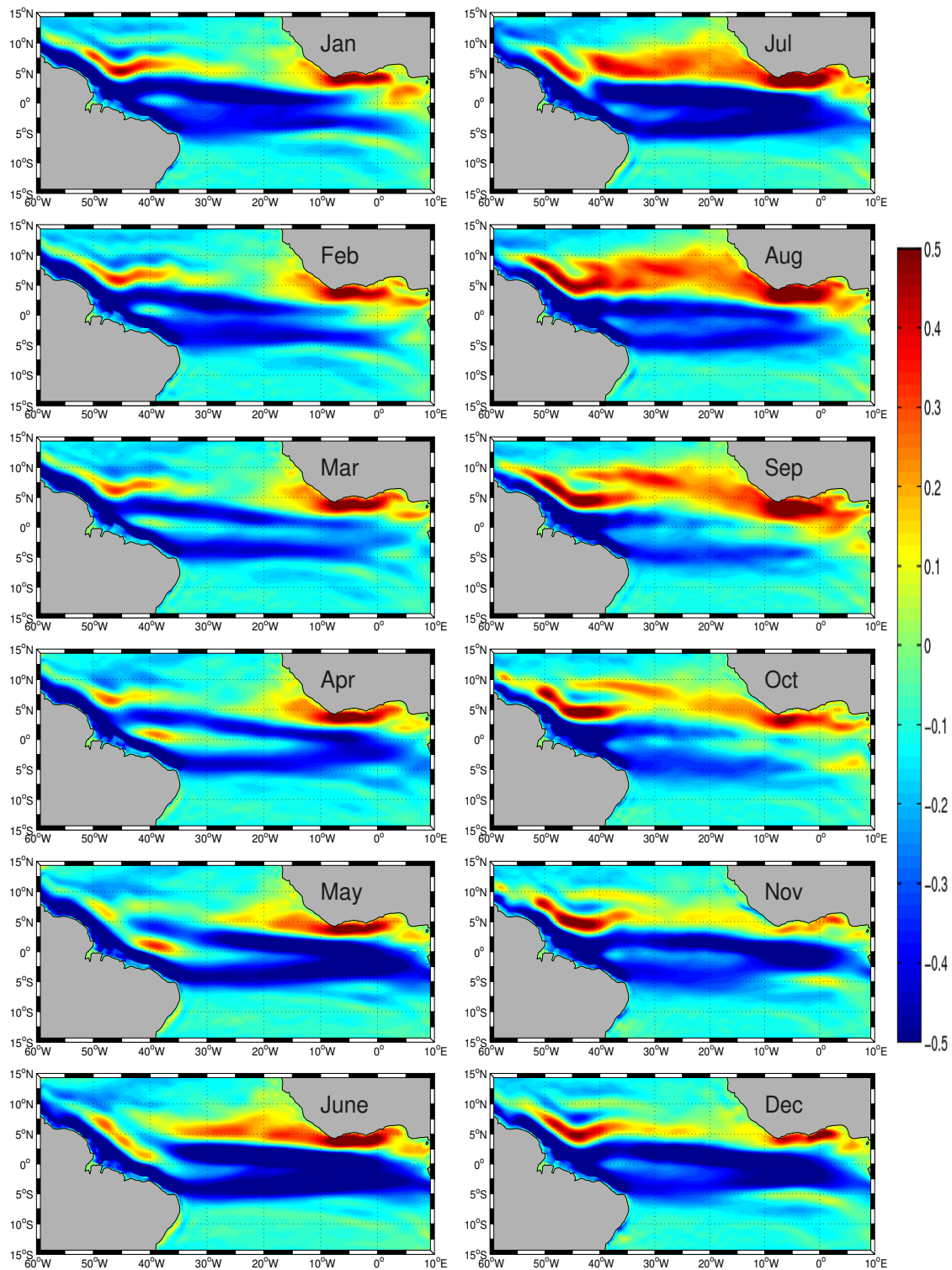
Figure 2. Model monthly climatology of zonal velocity at the ocean surface [ m s^{-1} ]. This figure should be compared with Fig. 6 in Rosell-Fieschi et al. (2015)
