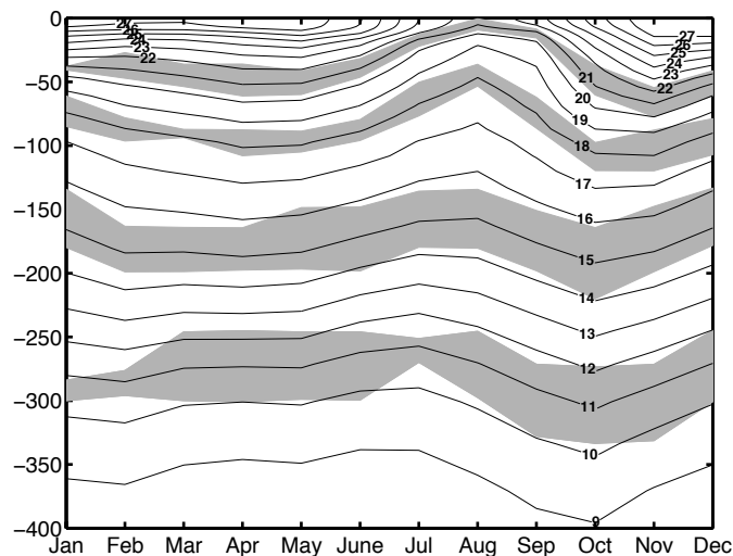
Figure 6. Time-depth representation of TROP025 climatological temperature [ ^{\circ} C] at 4^{\circ} N- 5^{\circ} W over the period 1982-2012. This figure should be compared with the climatological cycle observed at the same location between 1957 and 1964 (Picaut, 1983, his Fig. 15b). To evaluate uncertainty twenty four model climatologies were computed using 8-year averaging periods as in the observations (with starting years going from 1982 to 2005); the shallowest and deepest positions of 4 isotherms (11, 15, 18 and 21^{\circ} C) over this ensemble are shown with gray filling and indicate the limited role played by interannual variability, particularly for the 18 and 21^{\circ} C isotherm.
