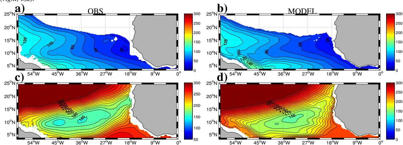
Figure 5. Depth [m] of the isopycnal density surface \sigma_t = 25.2 (top; a-b) and \sigma_t = 26.7 (bottom; c-d) in CORA (left; a,c) and TROP025 (right; b,d).
