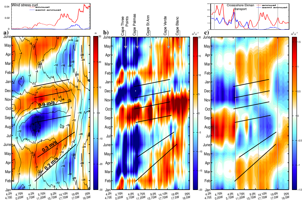
Figure 12. Time-alongslope distance diagram following the 100 m isobath (see location in Fig. 1) for the TROP025 climatological seasonal cycle of a) depth anomaly of the 18^\circ isotherm \delta z_{18} (colors, [m]) and SLA (contours, [cm]), (b) along-slope geostrophic transport between \sigma_t = 26.7 and the surface V_g^{26.7} [ m^2 s^{-1} ] c) across-shore Ekman transport anomaly. Oblique solid black lines correspond to propagation speeds of 0.2-0.3 (Feb.-June) and 0.9 ms^{-1} (Aug.-Jan.). They are subjectively drawn in panel a (and repeated in panels b and c) to indicate where spatio-temporal patterns are suggestive of alongslope propagation. In panel c, vertical gray lines delineate the sectors over which sector upwelling indices are computed (see Fig. 13). Power spectral densities associated with the annual and semi-annual harmonics of the wind stress curl and cross-shore Ekman transport along the 100 m isobath are displayed above panels a and c respectively.
