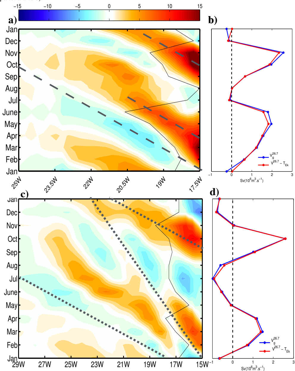
Figure 8. a,c): time-longitude diagram of vertically integrated meridional transport [ \text{m}^2 \text{s}^{-1} ] averaged along-slope between 13^\circ and 15^\circ \text{N} (a) and between 7^\circ and 9^\circ \text{N} (c). Propagation speed at 3.5 \text{ cm s}^{-1} (resp. 7.4 and 3 \text{ cm s}^{-1} ) are shown with dashed lines in panel a (resp. panel c). These values are the ones we choose as most appropriate to describe the propagation of patterns in the diagrams. b,d): associated climatologies of meridional transport integrated vertically and across-shore. Vertical integration is performed from the isopycnal surface \sigma_\theta = 26.7 up to the bottom of the mixed layer (left panel and red curve in right panel) or up to the surface but excluding Ekman transport, i.e., we only take into account the geostrophic flow (blue curve in right panel). Across-shore integration is performed from the shoreline to the first location where vertically integrated transport vanishes with a maximum longitude range of 3^\circ (integration limit is indicated with the thin solid line in panel a and c).
