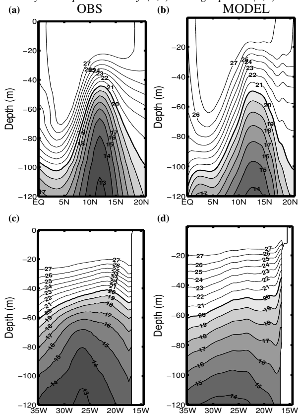
Figure 3. Meridional (resp. zonal) section at 26^{\circ}\text{W} (top, a-b) (resp. 13^{\circ}\text{N} ; bottom, c-d) for temperature [ ^{\circ}\text{C} ] averaged during september-october. Observations and models respectively correspond to the left (a,c) and right panels (b,d).
