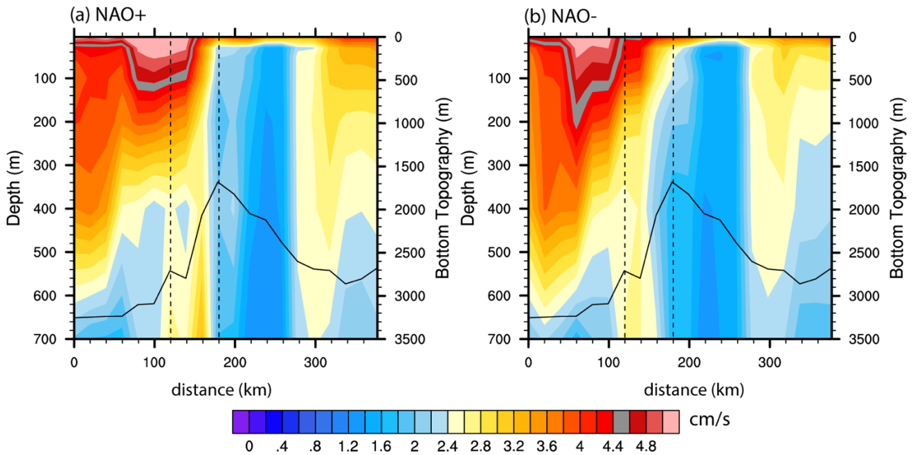
Figure 10: Composite of currents speed (cm/s) along the hydrographic section across the Mohn Ridge during (a) NAO+ and (b) NAO-. The dashed vertical lines show the position of the core of the AF.
