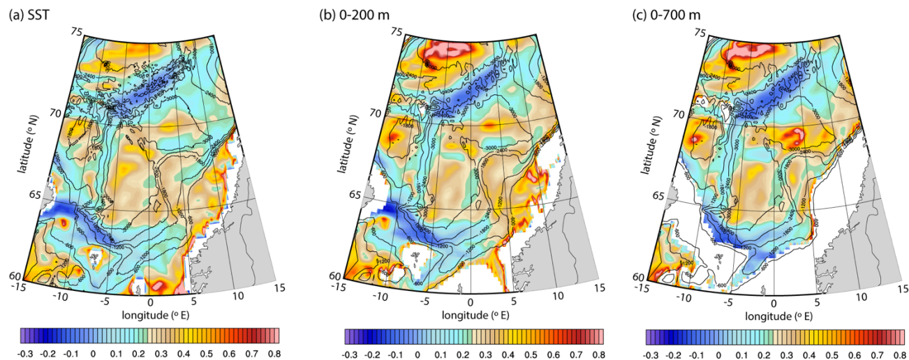
Figure 5: Singularity exponents estimated from TOPAZ (a) SST, (b) upper 200 m and (c) upper 700 m depth averaged potential temperature for the time period 1991-2015. Black isobaths are drawn for every 600 m. Regions shallower than 200 m and 700 m are masked respectively in panels b and c.
