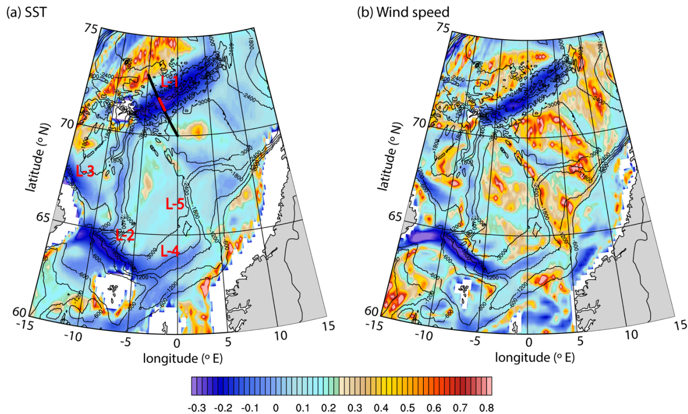
5 Figure 4: Singularity exponents estimated from the climatological mean (2002-2009) (a) AMSRE SST and (b) QuikSCat wind Speed. Black isobaths are drawn for every 600 m. In panel a, the bold black line shows the location of the vertical section across the Mohn Ridge shown in Figures 7, 8 and 10. The position of the core of the AF shown in Fig. 7 is marked as red over the bold black line. Locations 1, 2, 3, 4 and 5 are represented respectively by L-1, L-2, L-3, L-4 and L-5.
