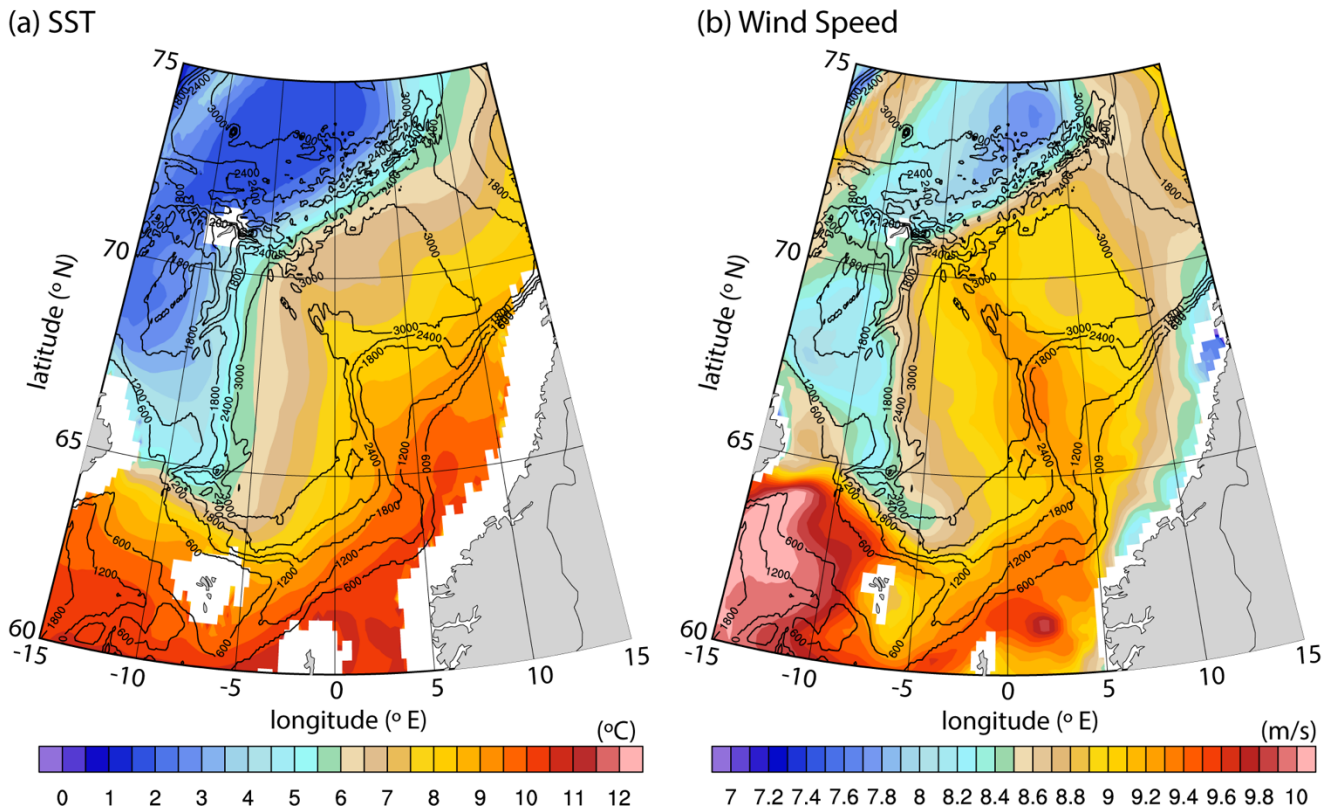
Figure 3: Climatological mean (2002-2009) (a) AMSRE SST ( ^{\circ}\text{C} ) and (b) QuikSCat wind speed (m/s). Black isobaths are drawn for every 600 m.
