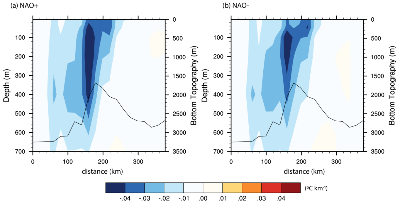
Figure 8: Gradient in the mean potential temperature ( ^{\circ}\text{C} / \text{km} ) along the hydrographic section across the Mohn Ridge during (a) NAO+ and (b) NAO-. The bottom topography along the section is indicated by the black contour.
