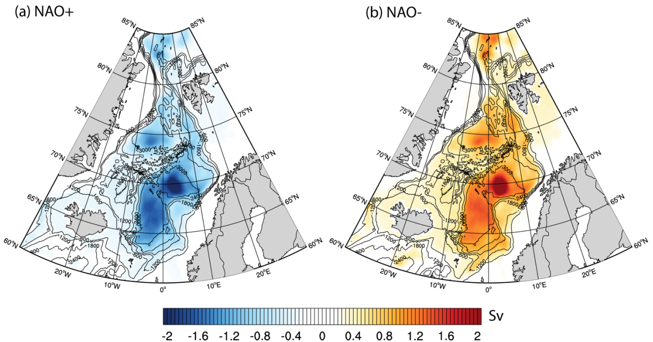
Figure 11: Composite map of anomalous BSFD, during (a) NAO+ and (b) NAO-. Black isobaths are drawn for every 600 m. Anomalies are computed using monthly climatology fields for the period 1991-2015.
