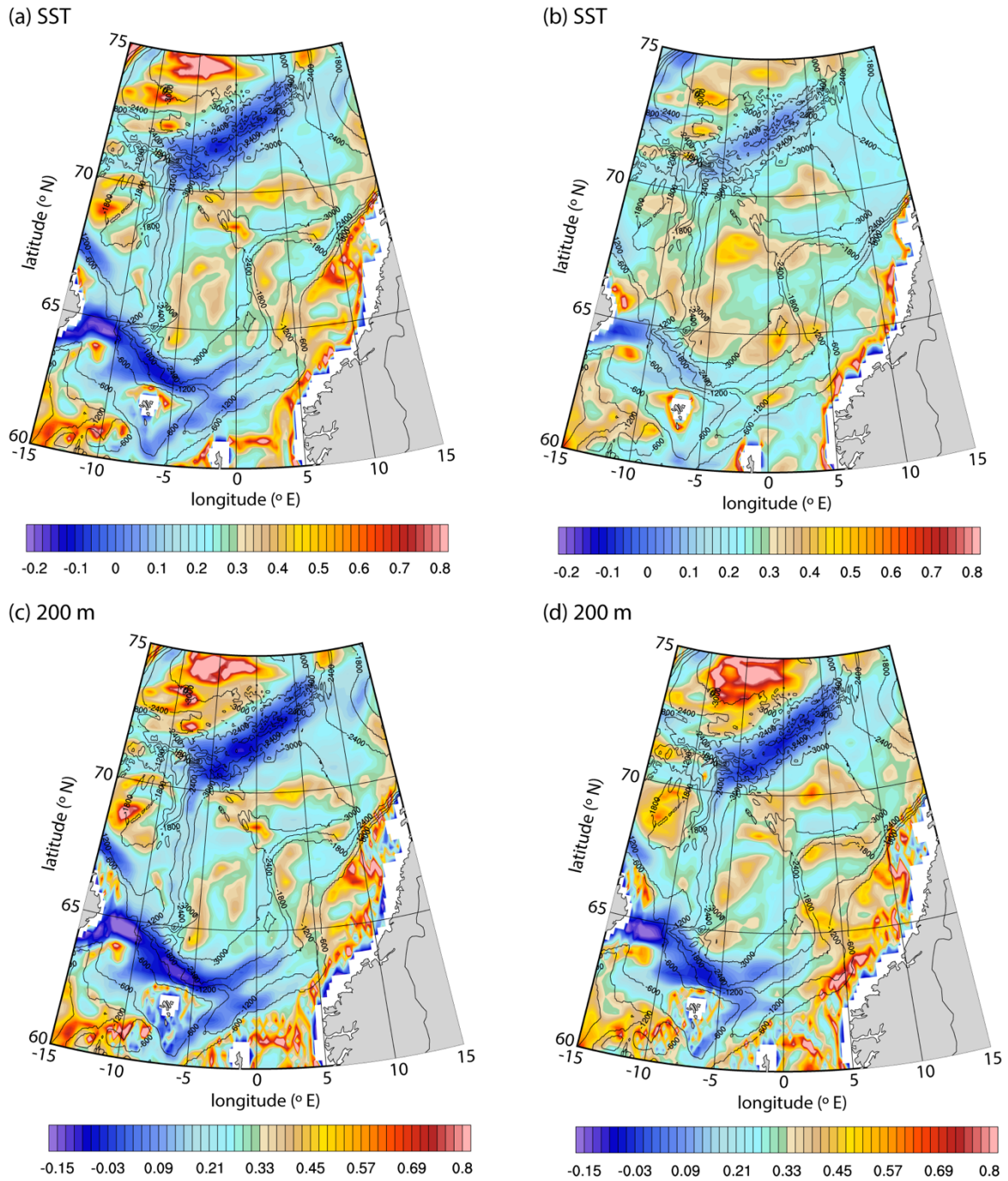
Figure 6: Singularity exponents estimated from TOPAZ (a-b) SST and (c-d) 200 m potential temperature for (a, c) winter (DJF) and (b, d) summer (JJA) for the time period 1991-2015.
