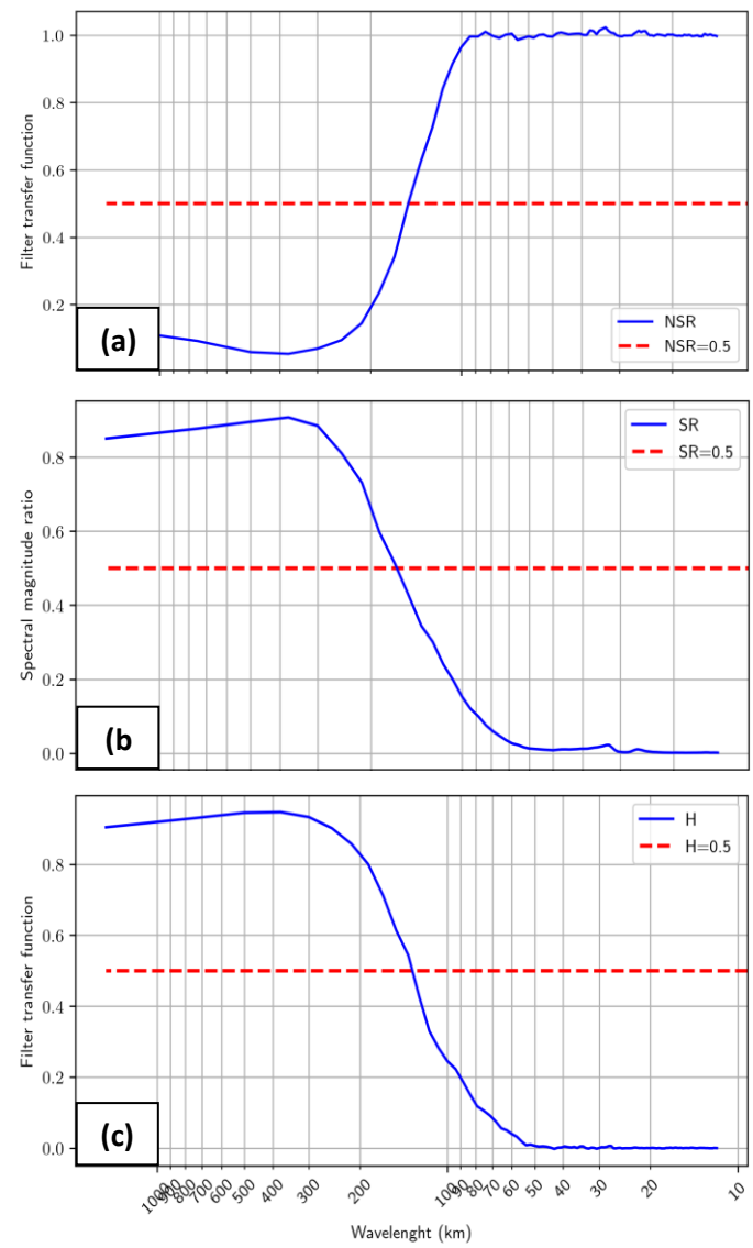
Figure A5: Illustration of the various spectral function used to estimate the resolution a 330°E, 45°N: a) with NSR method, b) with SR method, and c) with the transfer function
